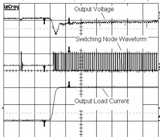
Load Transient Test ( V_{IN}=5V , V_{OUT}=1.2V , I_{OUT}=0A to 2A , PSAVE Mode Enabled, L_{OUT}=1.3\mu H , C_{OUT}=2\times 22\mu F , Channel 1: 50mV/Div, Channel 2: 5V/Div, Channel 4: 1A/Div, Time: 10μs/Div)
