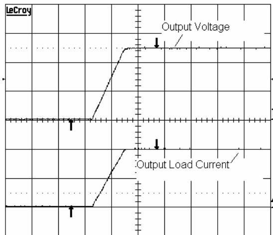
Load Transient Test (V IN =5V, V OUT =1.2V, I OUT = 0A to 2A, Forced Continuous Conduction Mode, L OUT =1.3μH, C OUT =2x22μF, Channel 1: 50mV/Div, Channel 2: 5V/Div, Channel 4: 1A/Div, Time: 10μs/Div)
