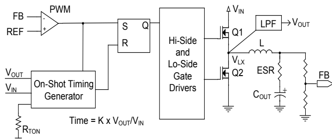
Figure 2 — On-Time Generation
