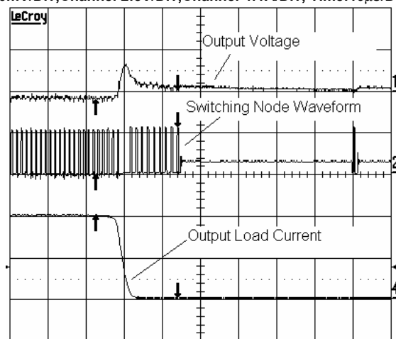
Load Transient Test ( V_{IN}=5V , V_{OUT}=1.2V , I_{OUT}=2A to 0A , PSAVE Mode Enabled, L_{OUT}=1.3\mu H , C_{OUT}=2\times 22\mu F , Channel 1: 50mV/Div, Channel 2: 5V/Div, Channel 4: 1A/Div, Time: 10μs/Div)
