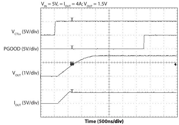
Start Up (CTL X ) — Full Load
