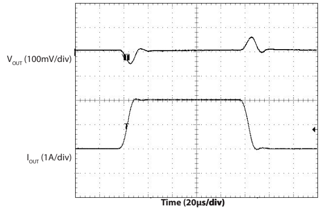
Transient Response ( V_{OUT} = 3.3V , I_{STEP} = 2A )
