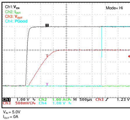
Start Up (CTL X ) — No Load
