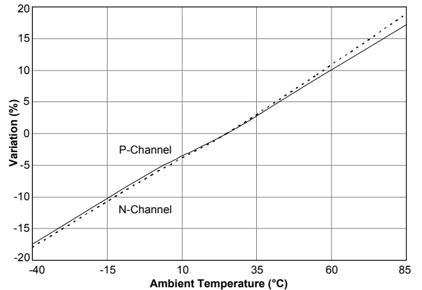
R_{DS(ON)} Variation vs. Temperature
