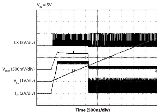
Start Up into Output Short Circuit
