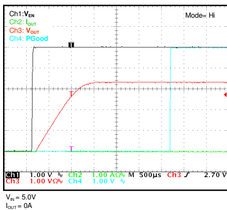
Start Up into Pre-Biased Output ( V_{OUT} = 1.5\text{V} )
