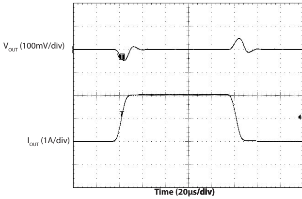
Transient Response ( V_{OUT} = 1.5V , I_{STEP} = 2A )
