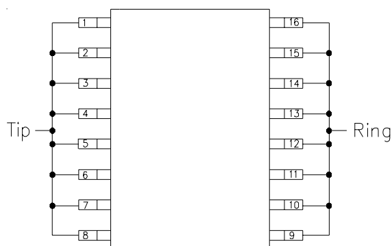
Figure 2 - Connection for Differential Protection (Line-to-Line)
