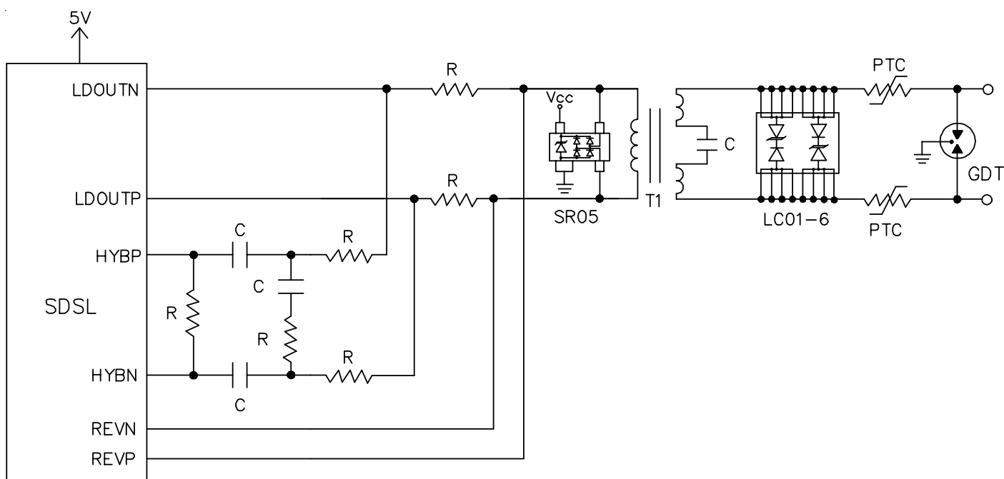
SDSL Protection
