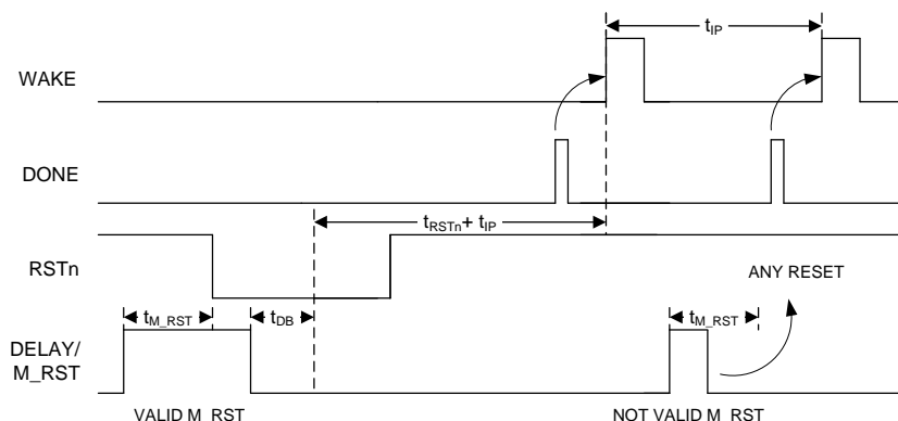
Figure 10. Manual Reset
