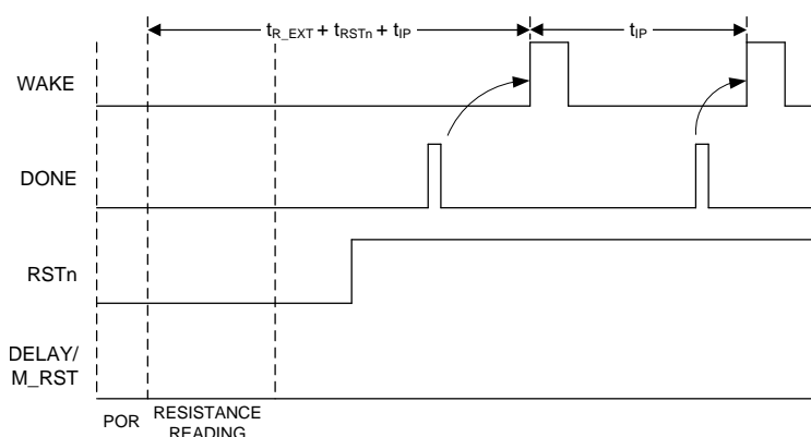
Figure 9. Startup
