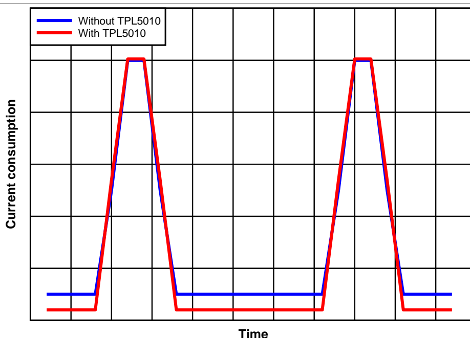
Figure 14. Effect of TPL5010 on Current Consumption
