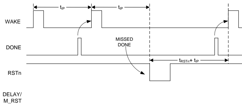
Figure 8. Watchdog
