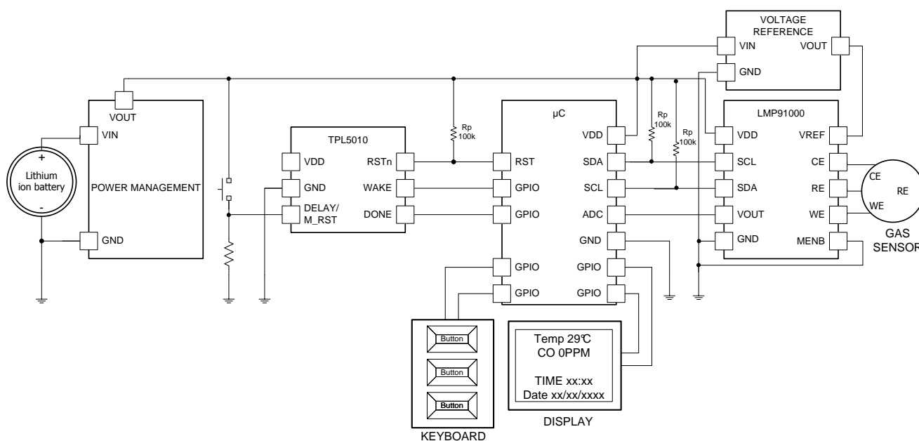
Figure 13. Data-logger
