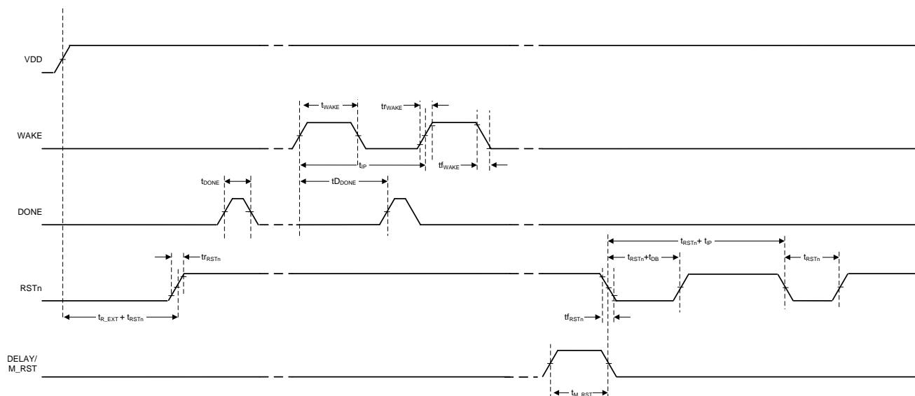
Figure 1. TPL5010 Timing
