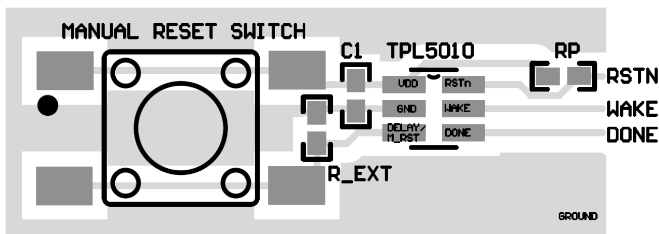
Figure 15. Layout
