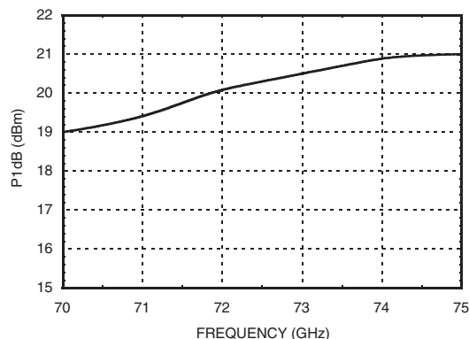
Fixtured Pout vs. Frequency
