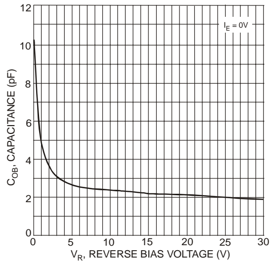
Fig. 4 Output Capacitance
