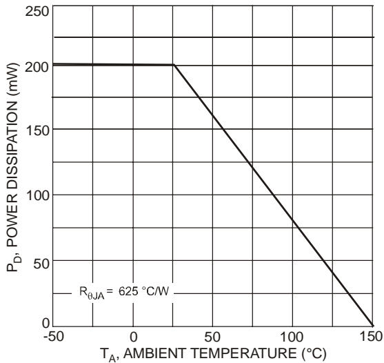
Fig. 1 Derating Curve
