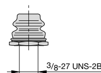
Knurled nut 3/8", plastic Y 307 117 02
