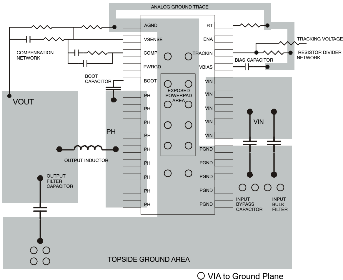
Figure 10. TPS54680 PCB Layout
