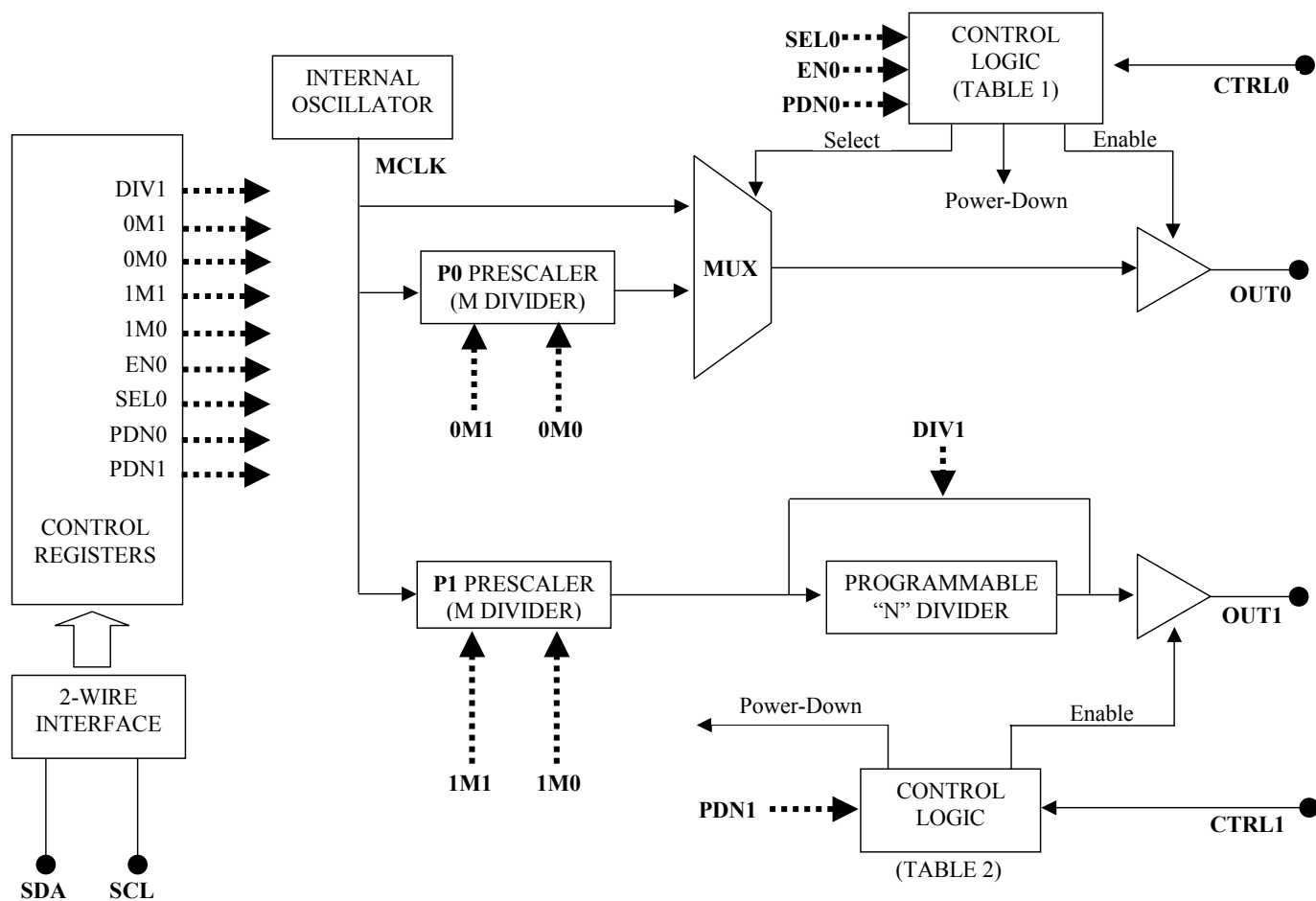
BLOCK DIAGRAM 1077 Figure1
