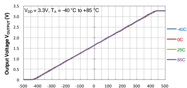
Output Voltage vs Magntic Flux Density
