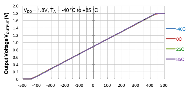
Output Voltage vs Magnetic Flux Density
