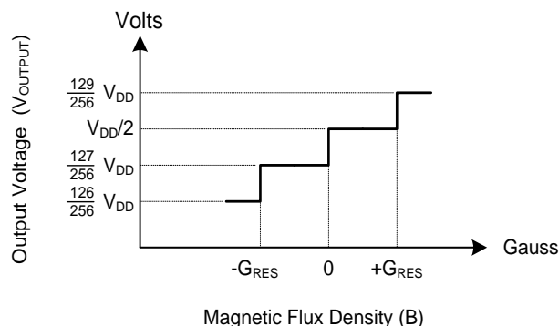
Transfer Curve Near 0 Gauss
