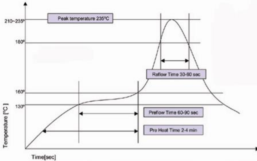
Figure 5 – Low Temperature Solder Reflow Thermal Profile
