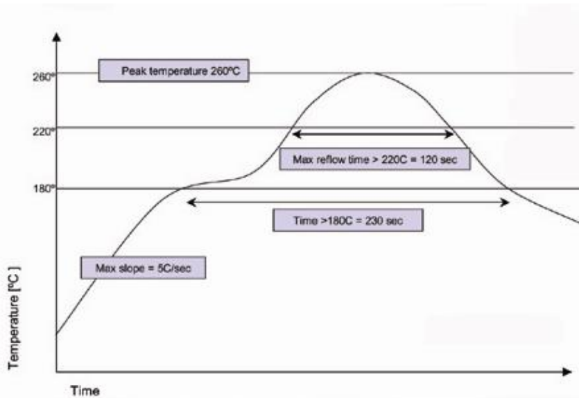
Figure 6 – High Temperature Solder Reflow Thermal Profile
