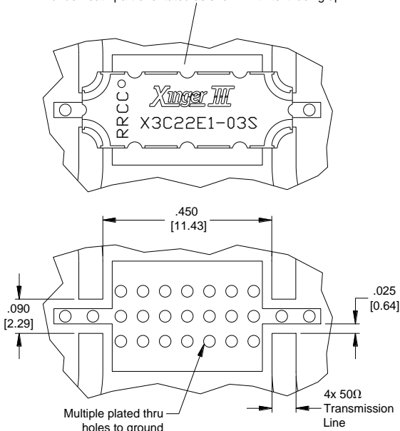
Dimensions Are in Inches [Millimeters] X3C22E1-03S Mounting Footprint
