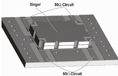
Figure 3: Component Placement
