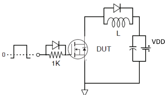
Fig 18. Gate Charge Test Circuit
