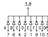
POLARITY DIAGRAM
