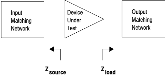
Figure 14. Series Equivalent Source and Load Impedance — 900 MHz
