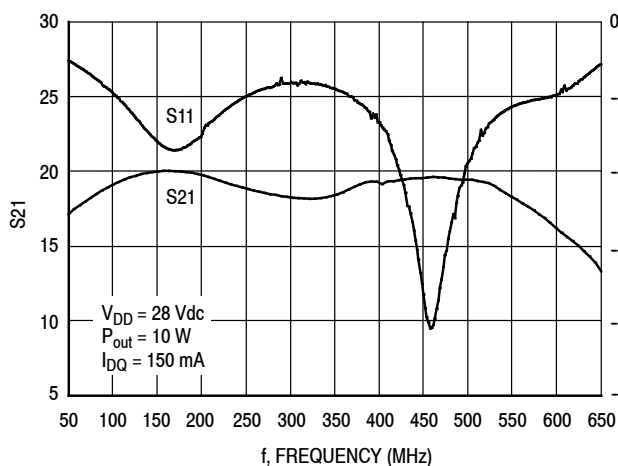
Figure 19. Broadband Frequency Response
