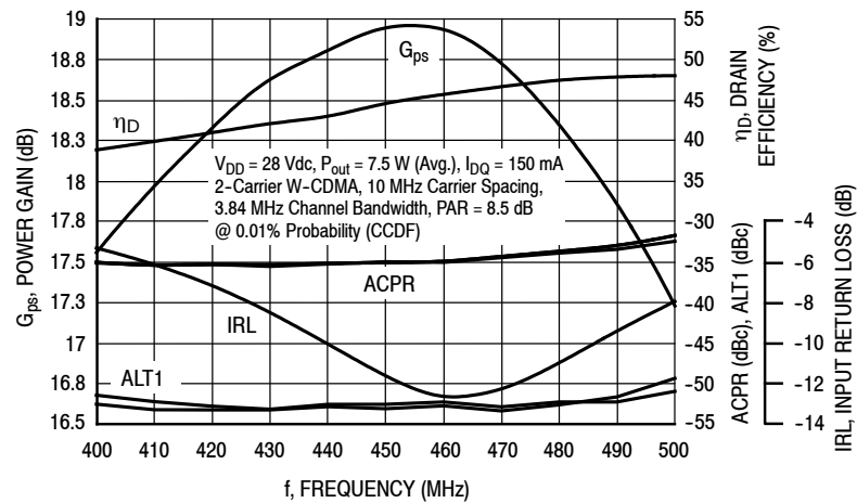
Figure 18. 2-Carrier W-CDMA Broadband Performance @ P_{out} = 7.5 Watts Avg.
