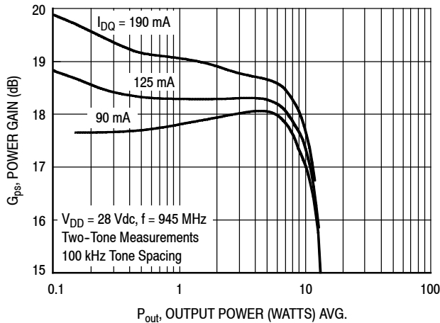
Figure 5. Two-Tone Power Gain versus Output Power
