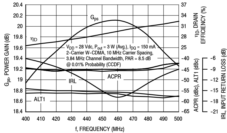
Figure 17. 2-Carrier W-CDMA Broadband Performance @ P_{out} = 3 Watts Avg.
