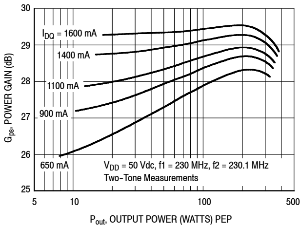
Figure 12. Two-Tone Power Gain versus Output Power
