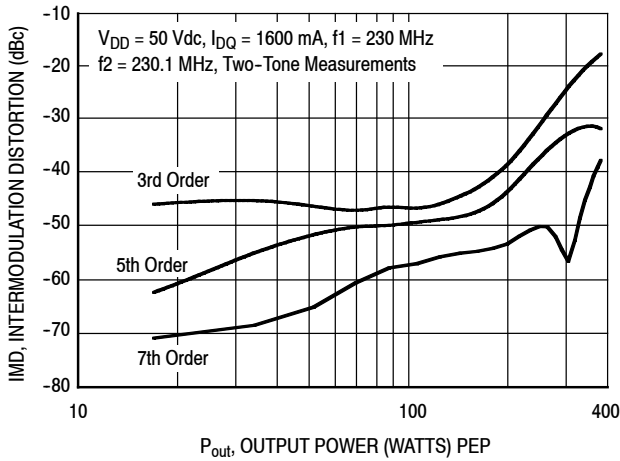
Figure 10. Intermodulation Distortion Products versus Output Power
