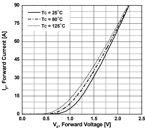
Fig 16. Typical Forward Voltage Drop vs. Forward Current - Rectifier Diode
