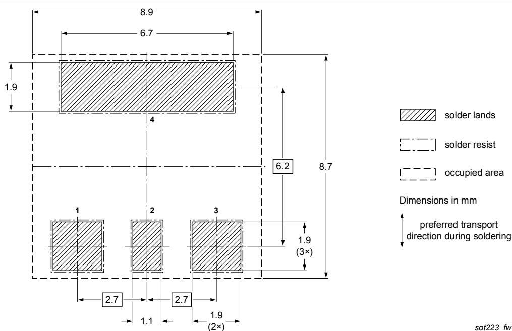
Fig. 13. Wave soldering footprint for SC-73 (SOT223)
