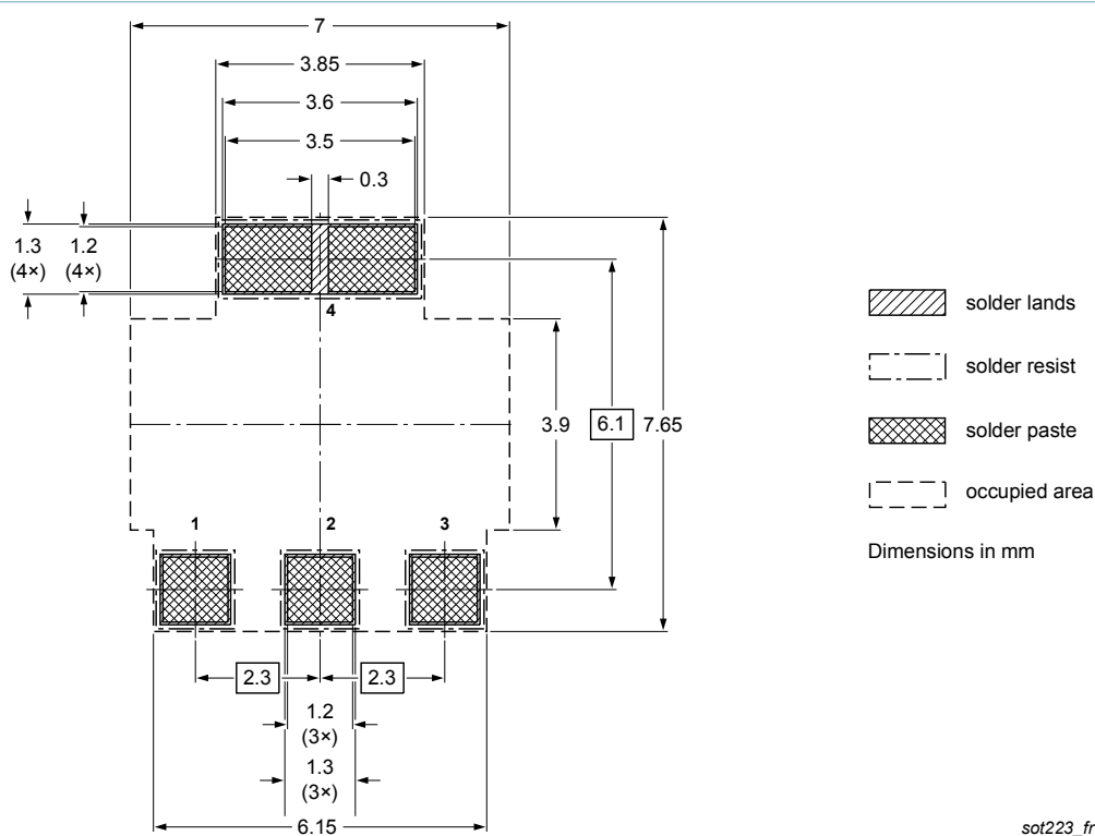
Fig. 12. Reflow soldering footprint for SC-73 (SOT223)
