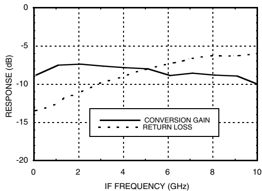
IF Bandwidth
