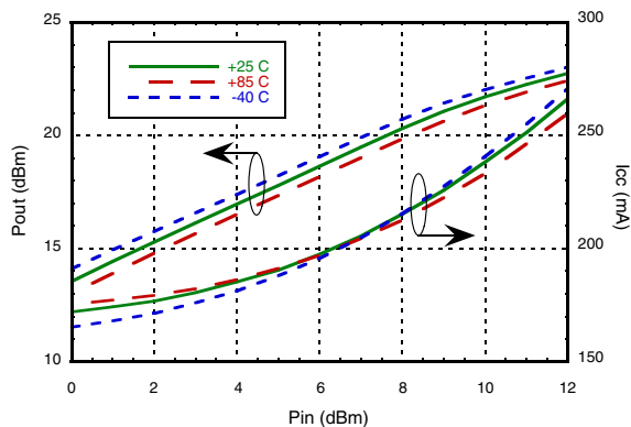
Pout & Icc vs. Temperature
