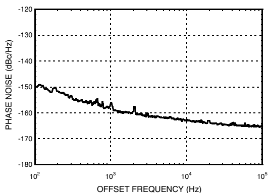
Phase Noise at Pout = +10 dBm @ 3 GHz
