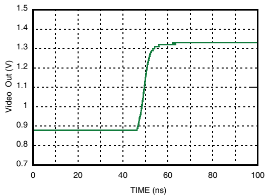
Rise Time @ 10 GHz @ -20 dBm
