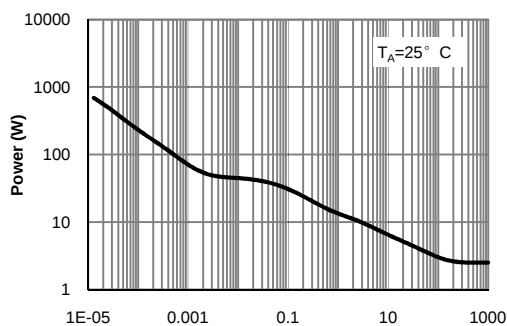
Figure 14: Single Pulse Power Rating Junction-to-Ambient (Note H)
