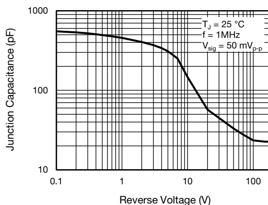
Fig. 5 - Typical Junction Capacitance Per Diode
