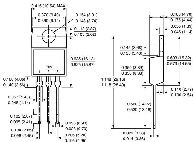
TO-220AB
