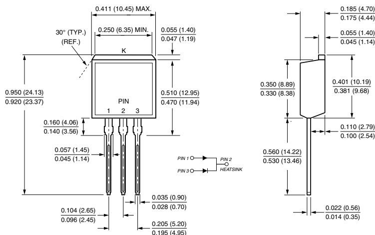
TO-262AA
