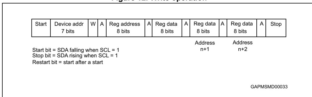
Figure 12. Write operation
