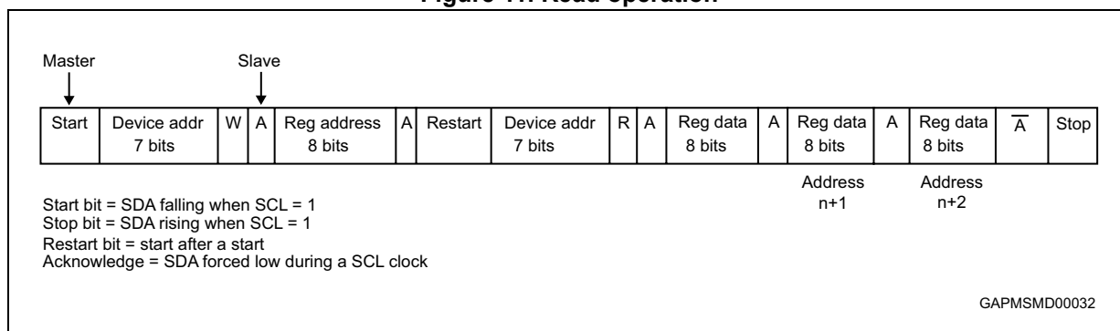
Figure 11. Read operation
