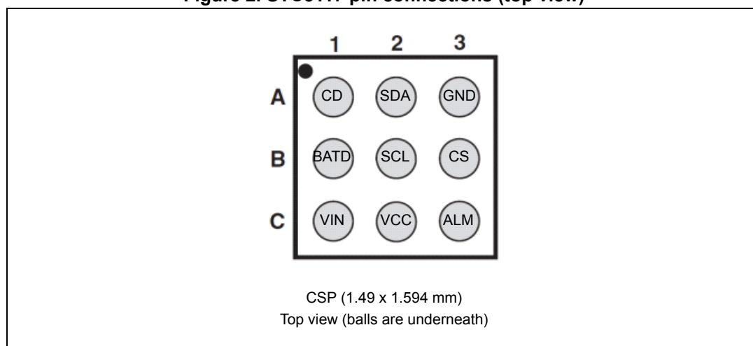
Figure 2. STC3117 pin connections (top view)
