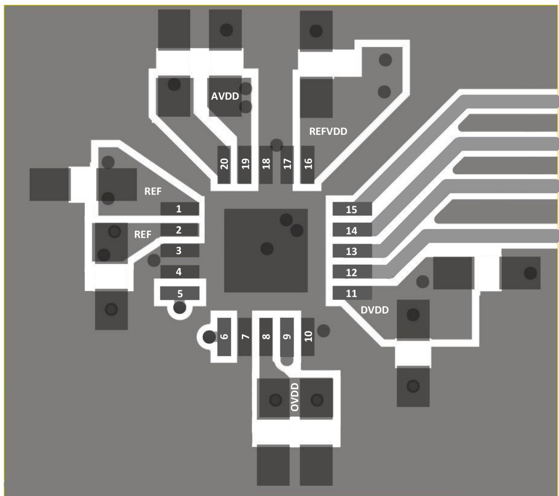
Figure 15. Top-Layer Sample Layout
