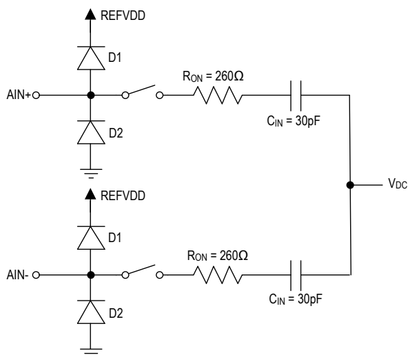
Figure 2. Simplified Model of Input Sampling Circuit
