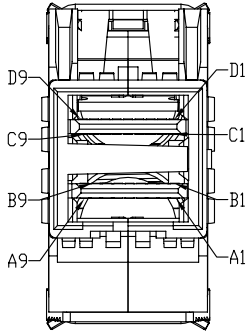
P1 VIEW A SCALE 4:1
