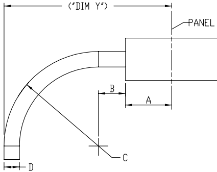
BEND RADIUS TOP VIEW OF CONNECTOR
