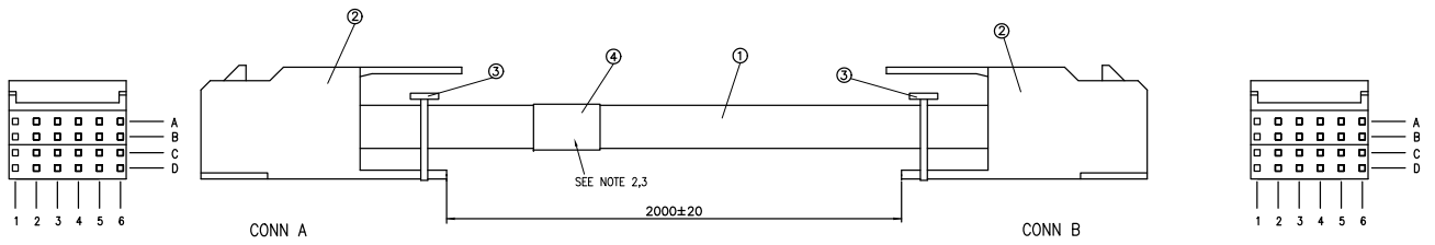
WIRE DIAGRAM
