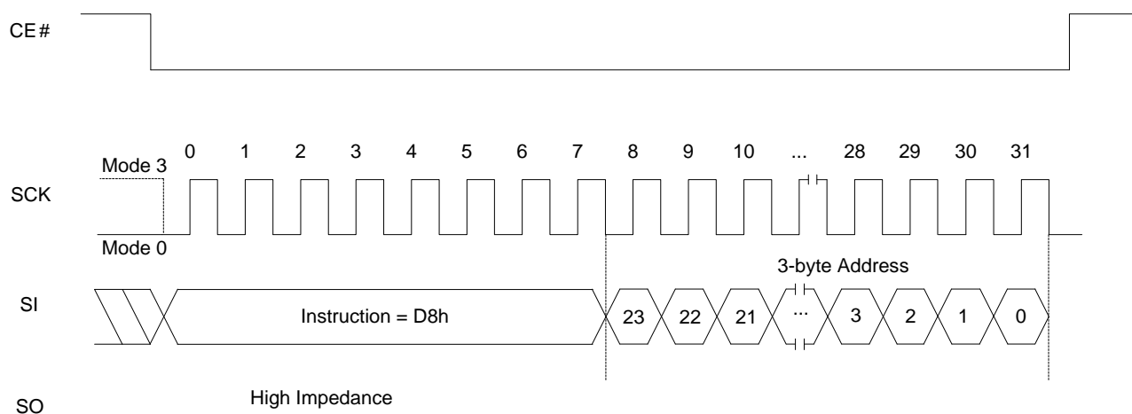
Figure 8.11 Block Erase (64KB) Sequence
