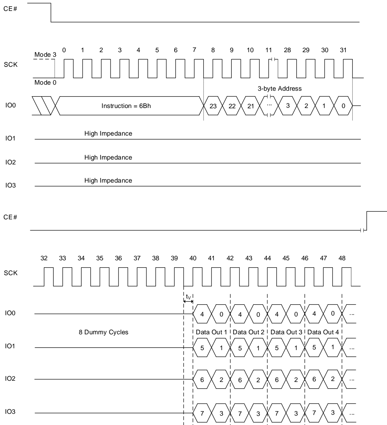
Figure 8.6 Fast Read Quad-Output Sequence
