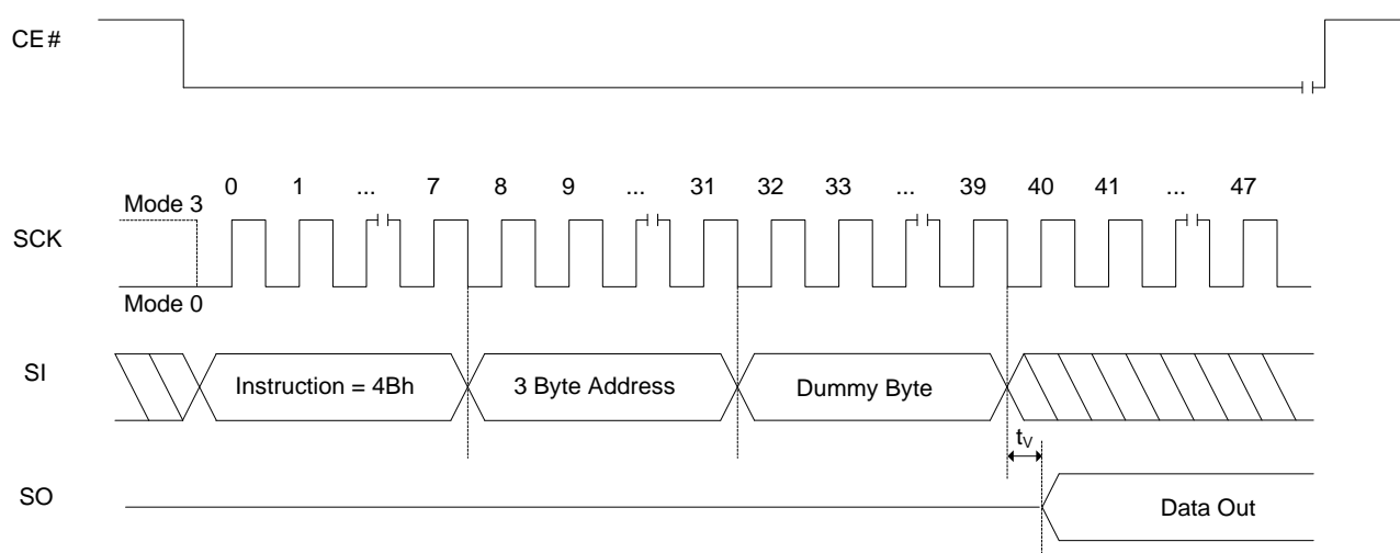
Figure 8.25 RDUID Operation
