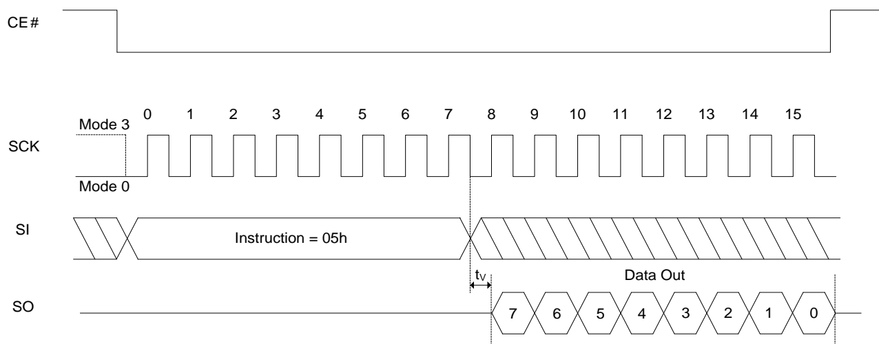
Figure 8.16 Read Status Register Sequence
