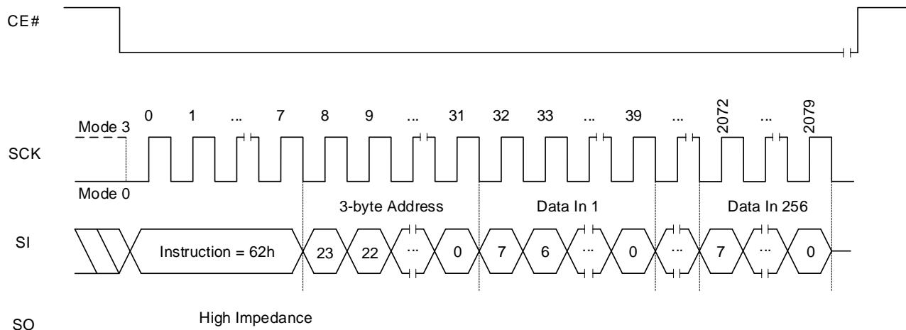
Figure 8.28 IRP (Information Row Program) Operation
