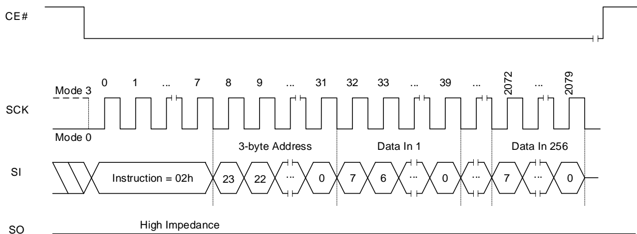
Figure 8.8 Page Program Sequence
