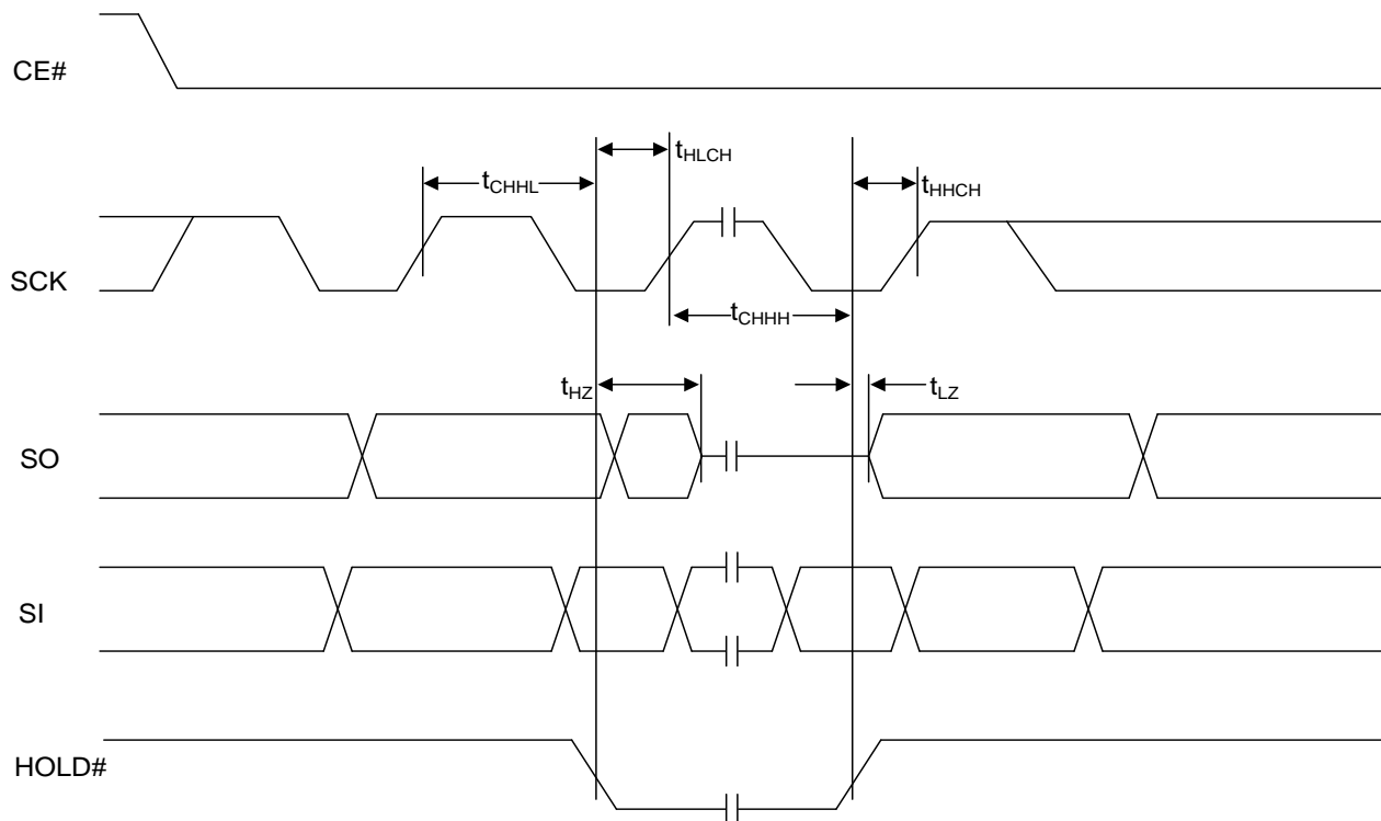
Figure 9.3 HOLD TIMING
