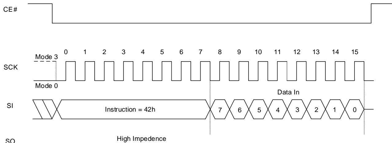
Figure 8.19 Write Function Register Sequence
