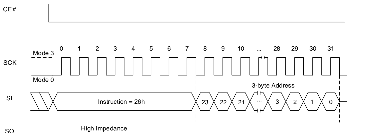
Figure 8.30 Sector Unlock Sequence
