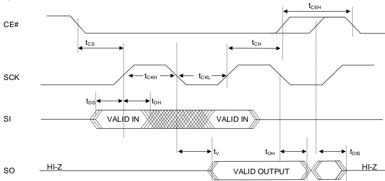
Figure 9.2 SERIAL INPUT/OUTPUT TIMING (1)
