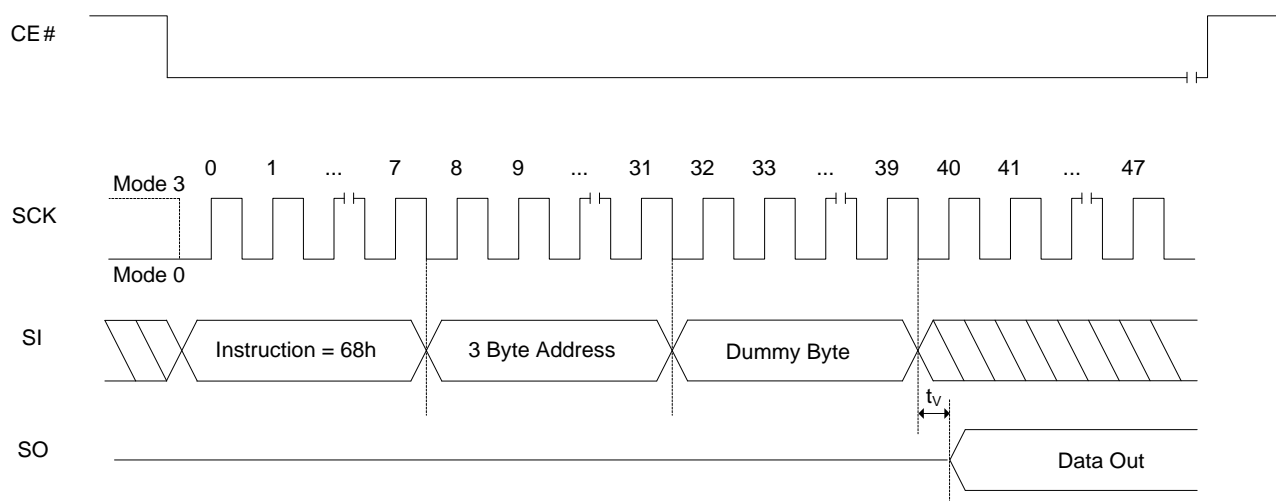
Figure 8.29 IRRD (Information Row Read) Operation
