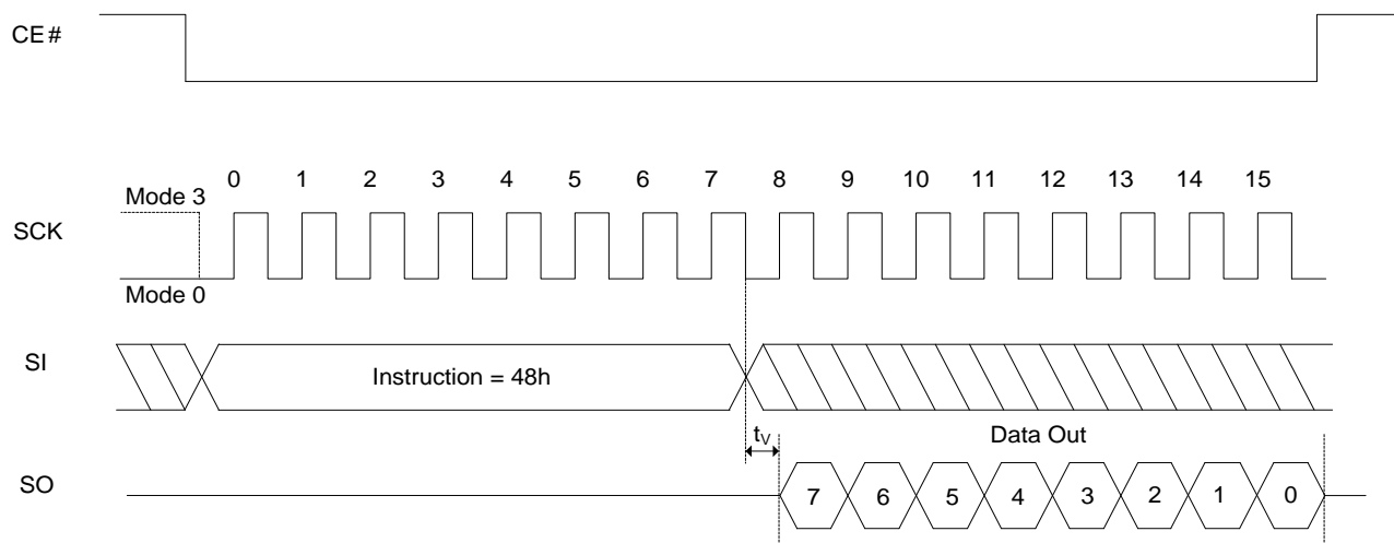
Figure 8.18 Read Function Register Sequence
