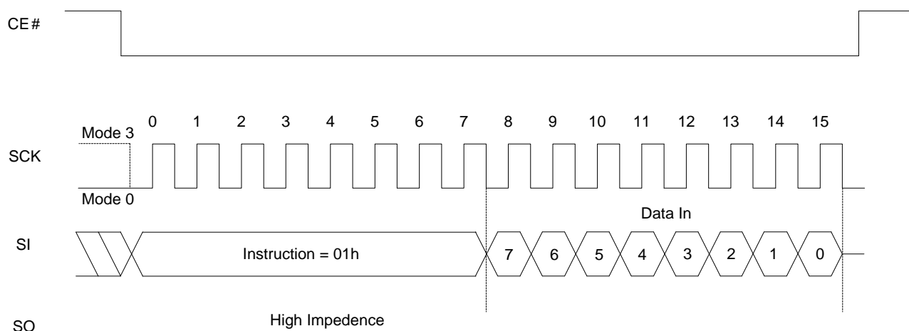
Figure 8.17 Write Status Register Sequence
