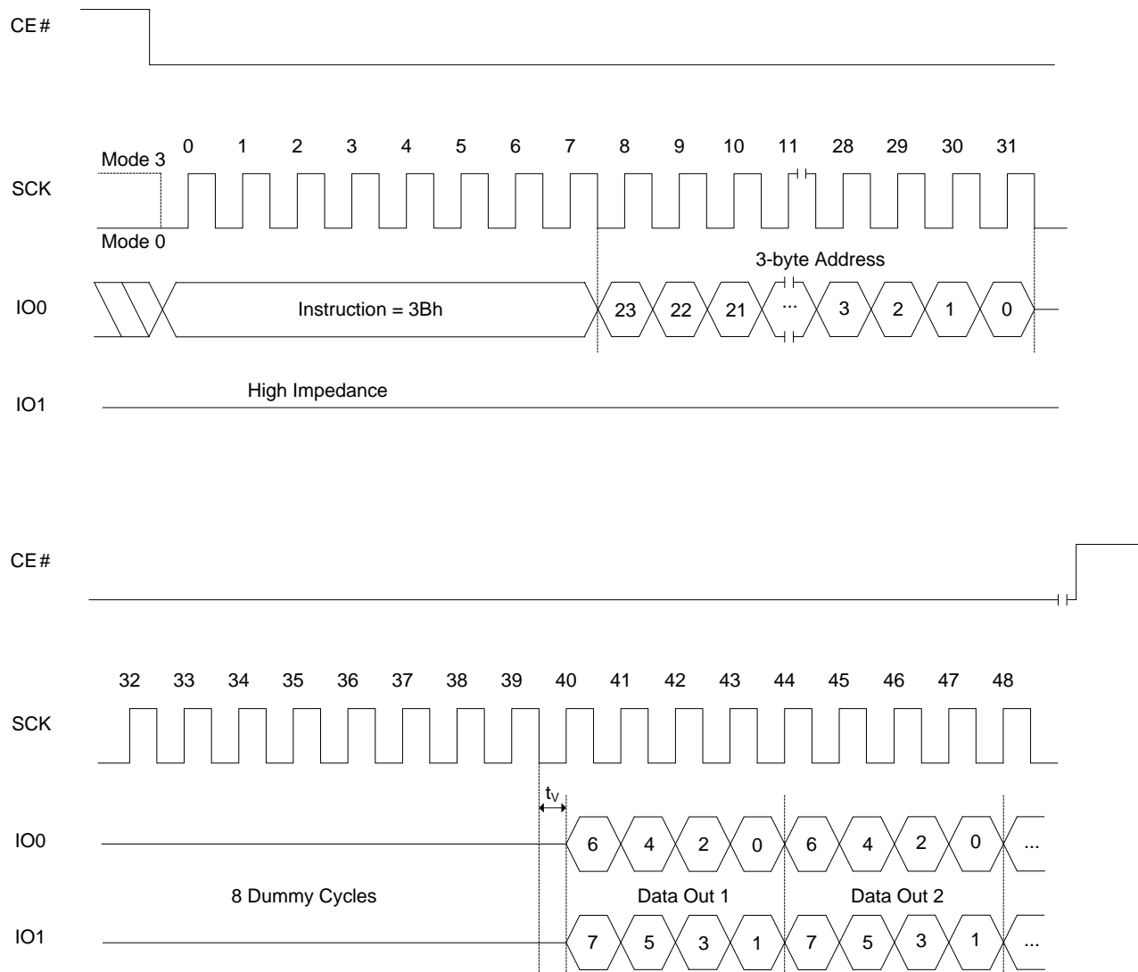
Figure 8.5 Fast Read Dual-Output Sequence
