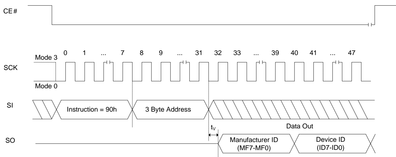
Figure 8.24 Read Product Identification by RDMDID Sequence
