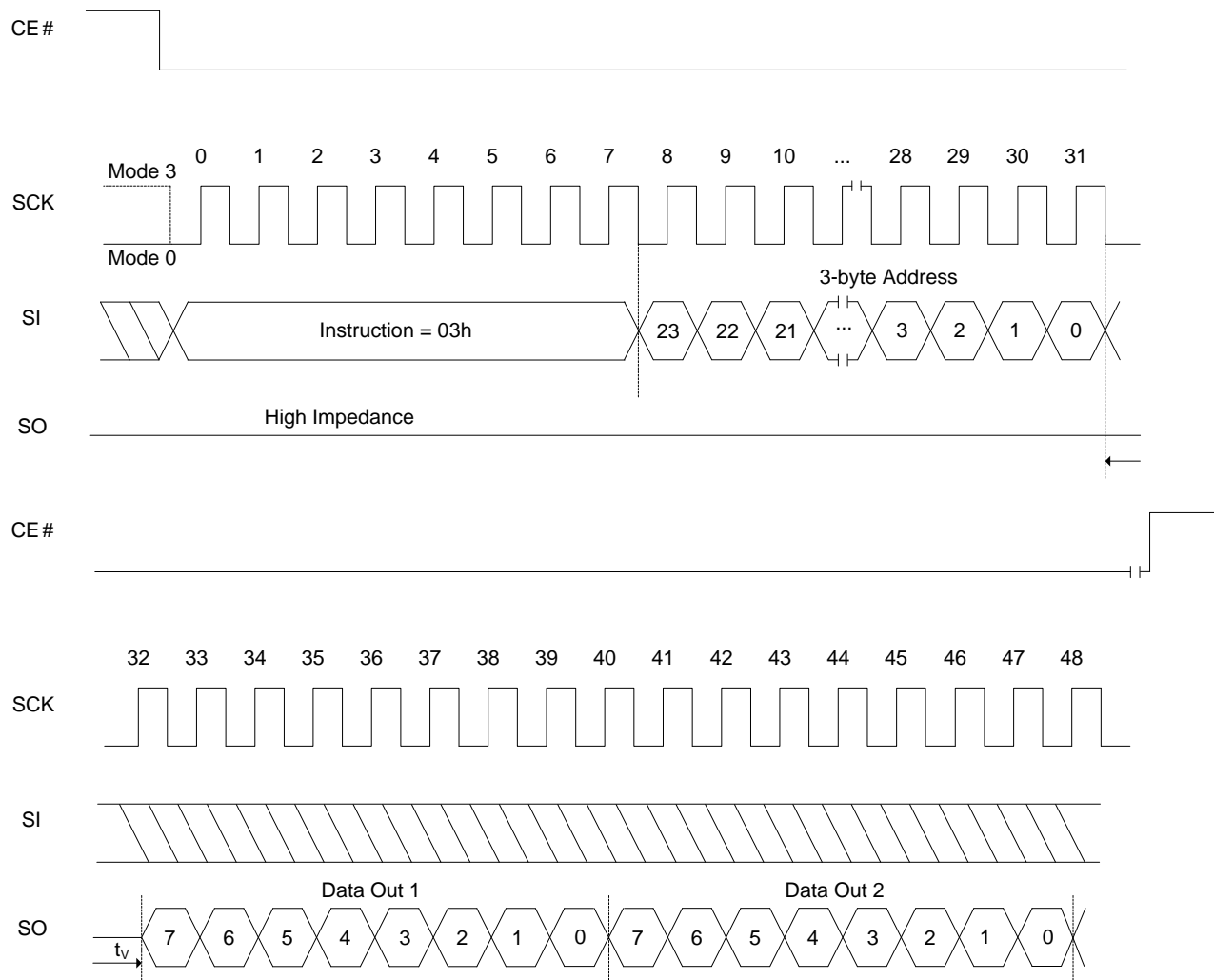
Figure 8.1 Read Data Sequence
