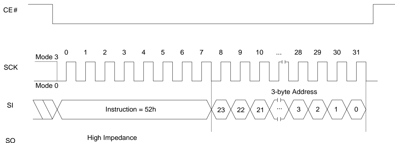
Figure 8.12 Block Erase (32KB) Sequence
