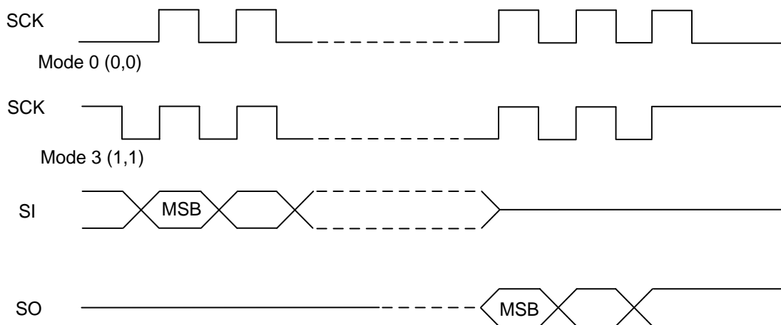
Figure 4.2 SPI Mode Support
