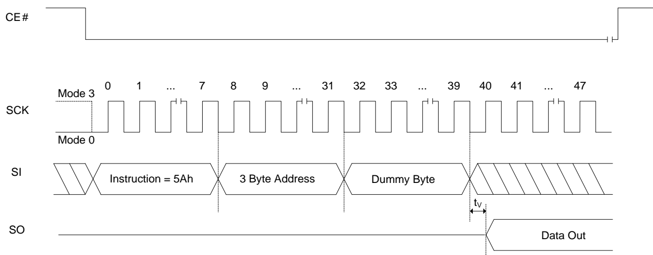
Figure 8.26 RDSFDP (Read SFDP) Operation
