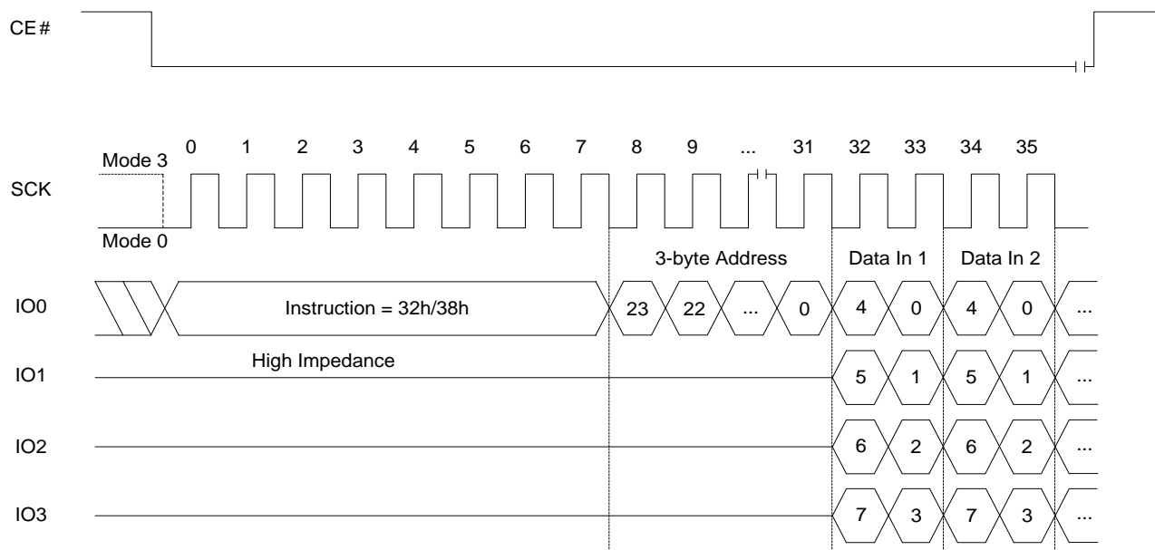
Figure 8.9 Quad Input Page Program operation
