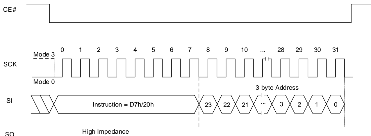
Figure 8.10 Sector Erase Sequence
