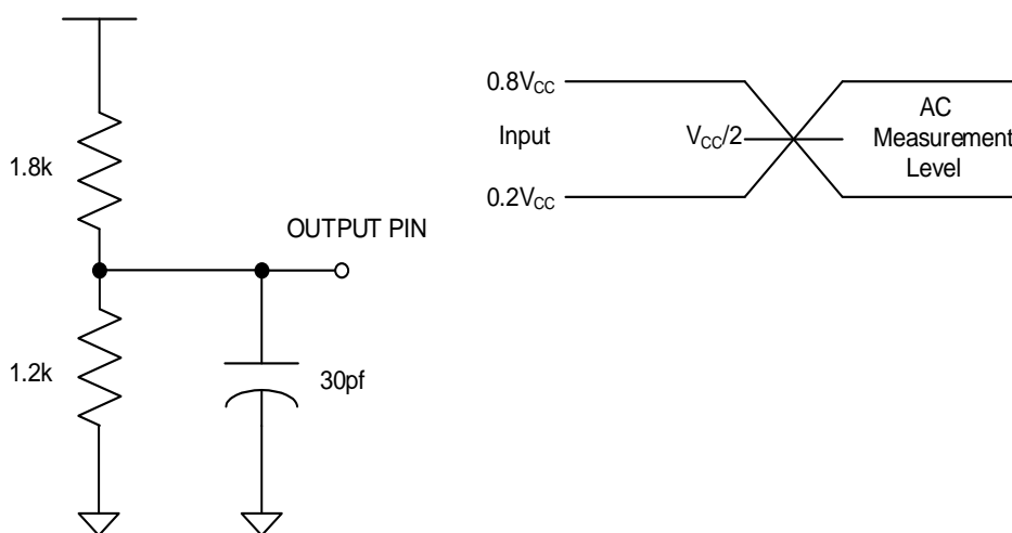
Figure9.1 Output test load & AC measurement I/O Waveform
