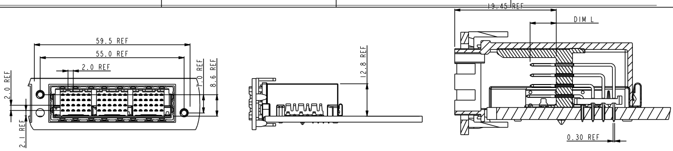
SECTION 1-1 SCALE 2.000
