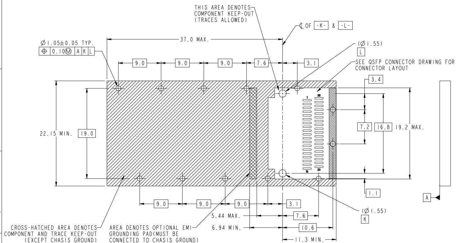
PCB LAYOUT FOR SINGLE SIDED APPLICATION
