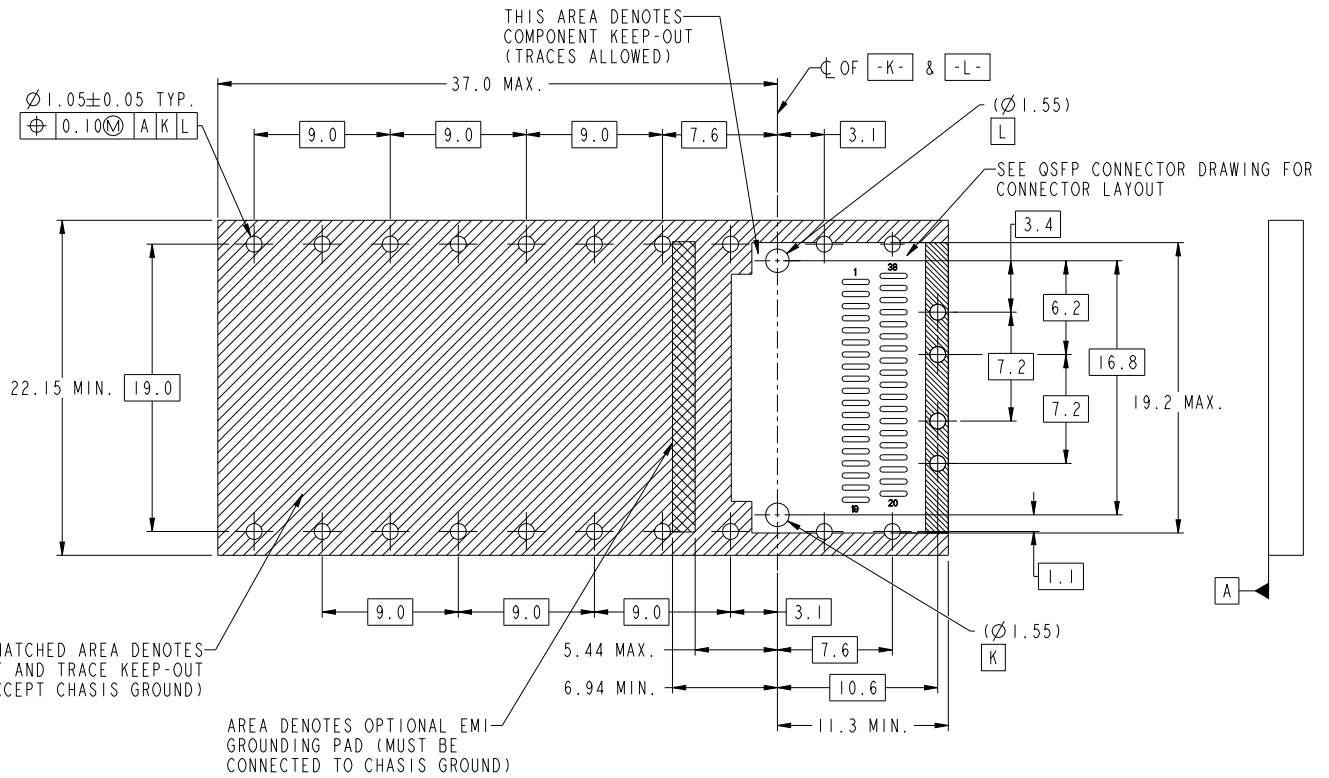
PCB LAYOUT FOR BELLY TO BELLY APPLICATION
