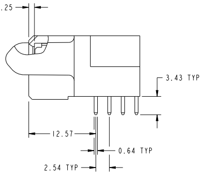
BROKEN-OUT SECTION B-B SCALE 2:1
