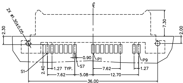
RECOMMENDED PCB LAYOUT PCB THICKNESS: 1.6mm
