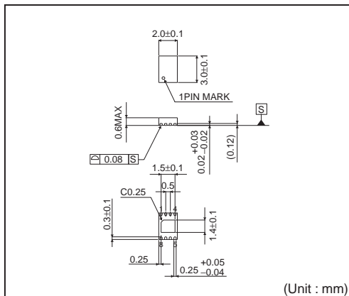
VSON008X2030
