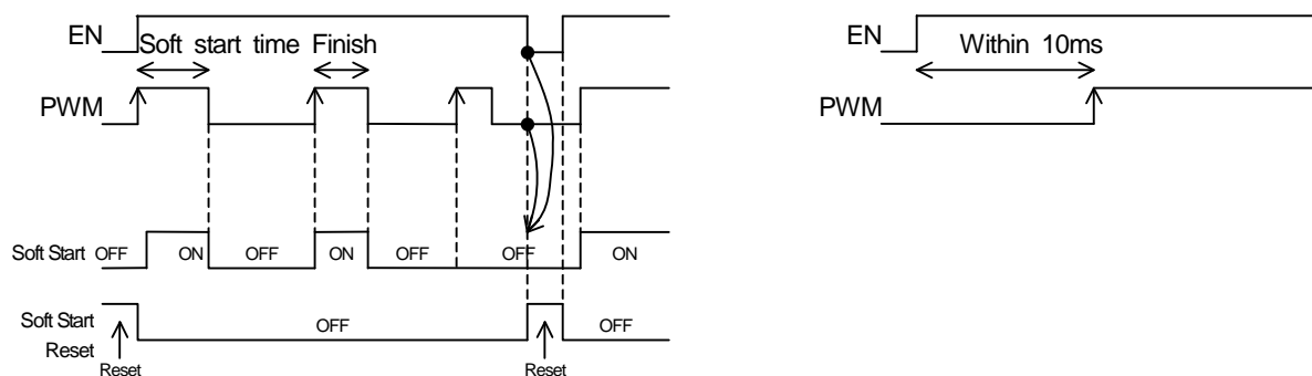
Figure 2. Soft start
