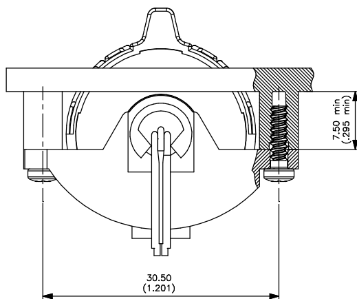
EXAMPLE OF MOUNTING
