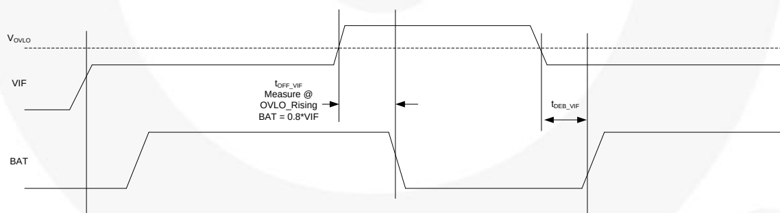
Figure 10. Timing for V_{IF} OVLO Operation (ON=Don't Care)
