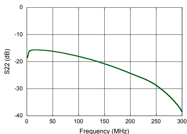
Output Return Loss with 15 dB Gain
