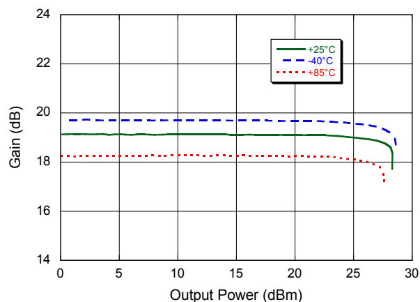
P1dB @ 250 MHz
