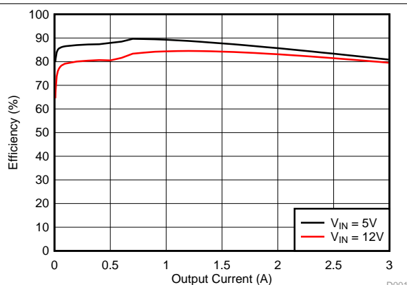
Figure 34. TPS563210 Efficiency
