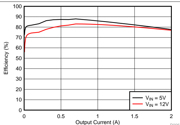
Figure 19. TPS562210 Efficiency
