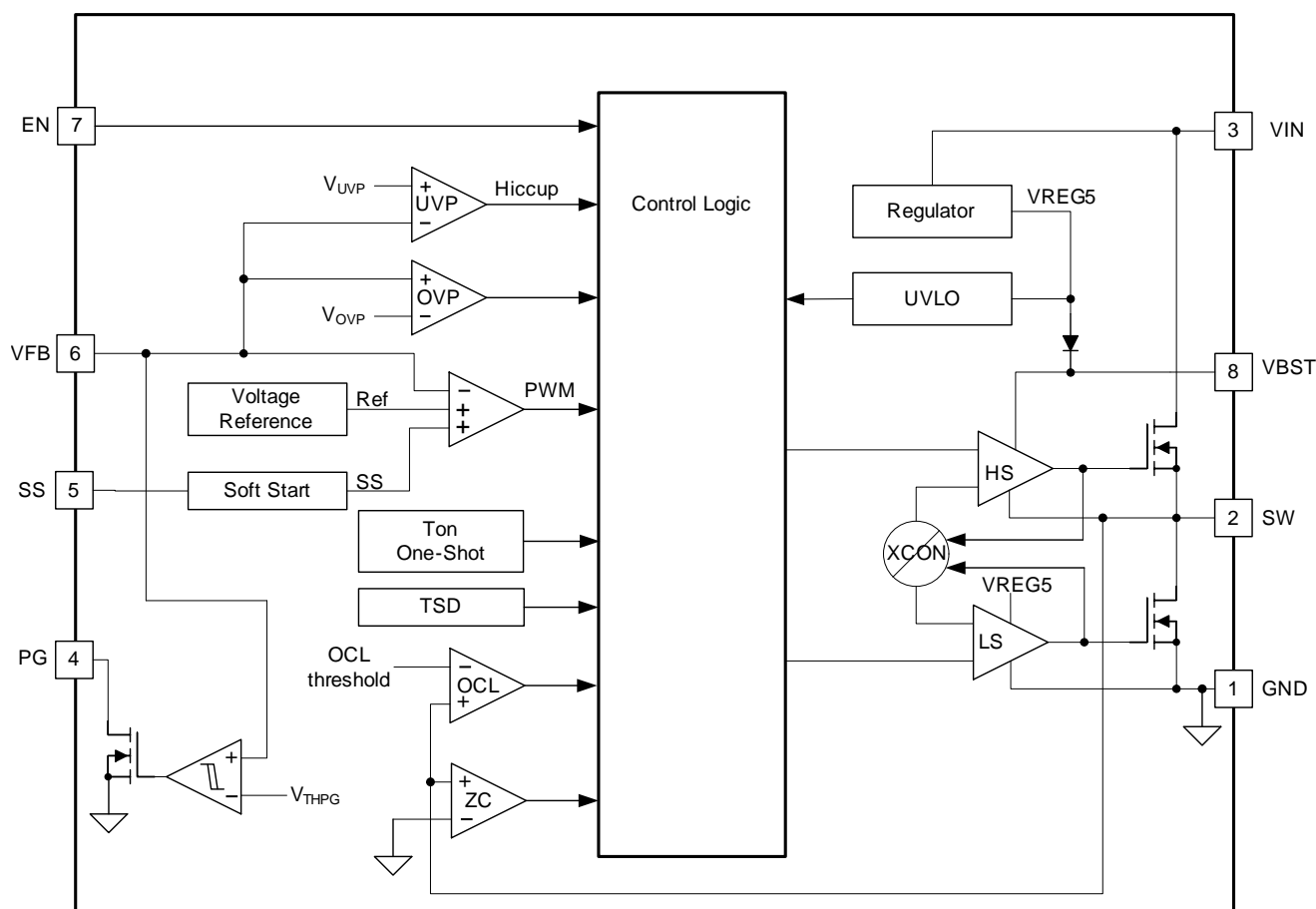
Figure 17. TPS562210
