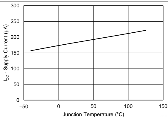
Figure 9. Supply Current vs Junction Temperature
