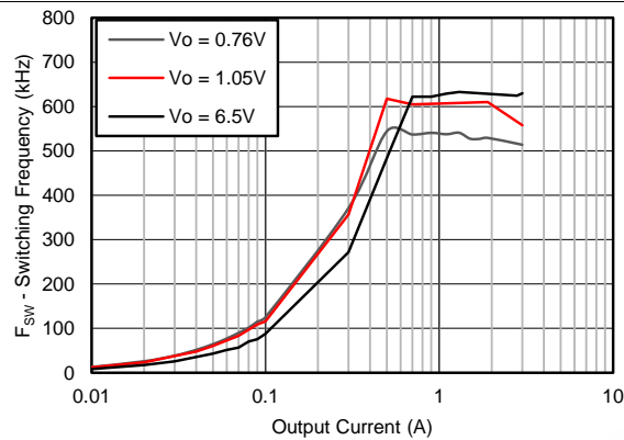
Figure 16. Switching Frequency vs Output Current
