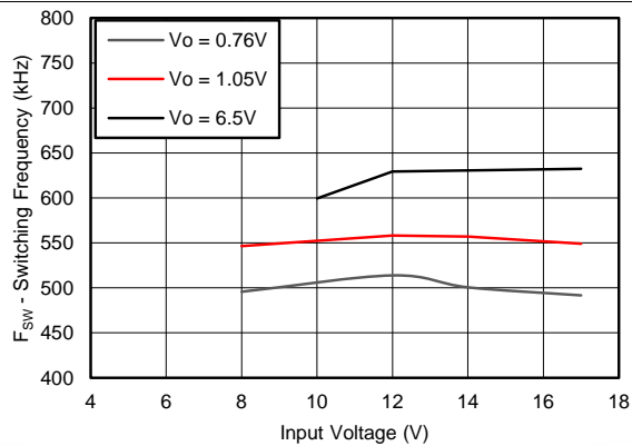
Figure 15. Switching Frequency vs Input Voltage
