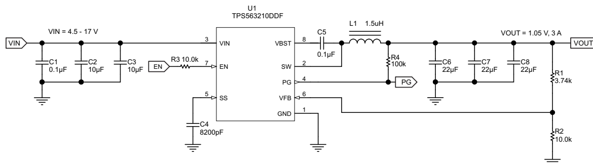
Figure 33. TPS563210 1.05 V / 3A Reference Design
