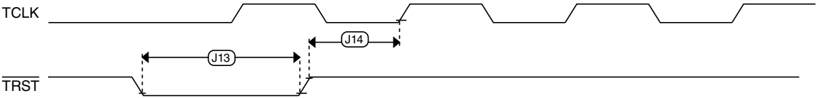
Figure 10. TRST timing
