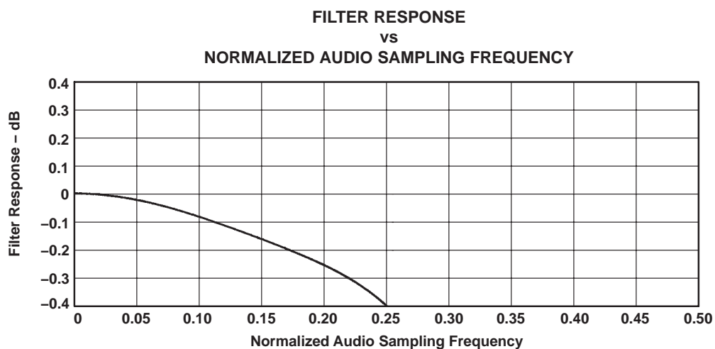
Figure 3-18. ADC Digital Filter Ripple 3: USB Mode Only
