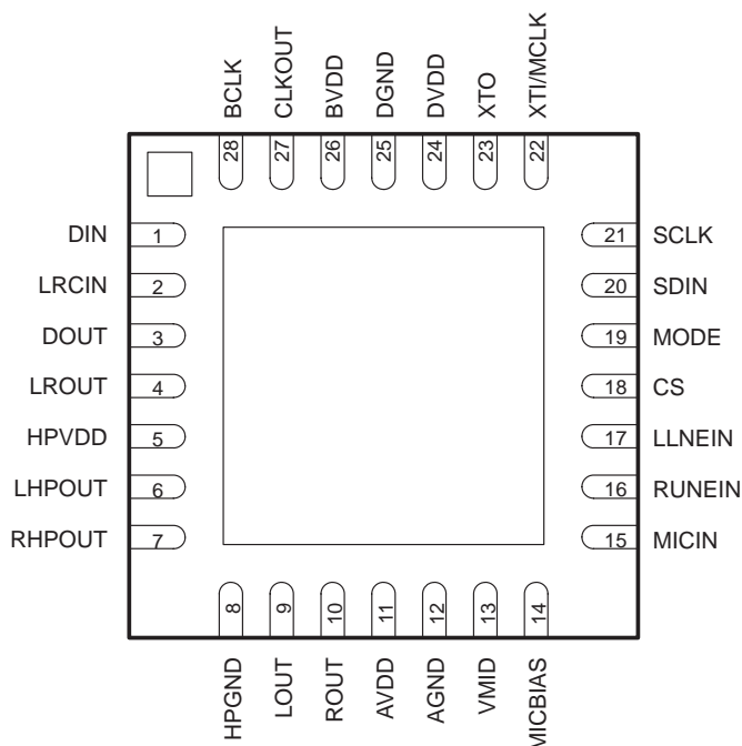
RHD PACKAGE (TOP VIEW)
