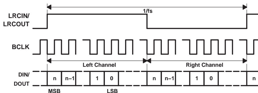
Figure 3-6. Left-Justified Mode Timing
