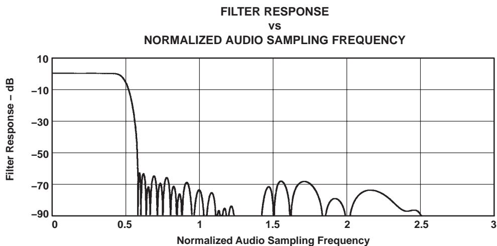
Figure 3-13. ADC Digital Filter Response 1: USB Mode Only
