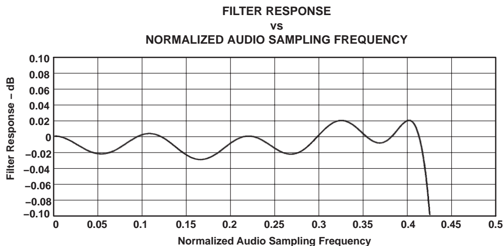
Figure 3–22. DAC Digital Filter Ripple 1: USB Mode Only
