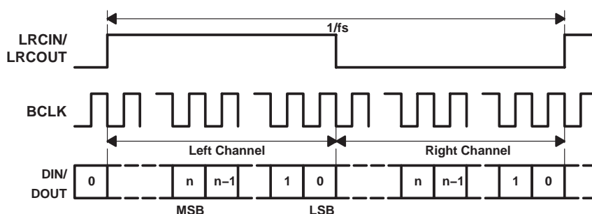
Figure 3-5. Right-Justified Mode Timing
