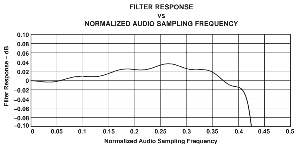
Figure 3-14. ADC Digital Filter Ripple 1: USB Mode Only
