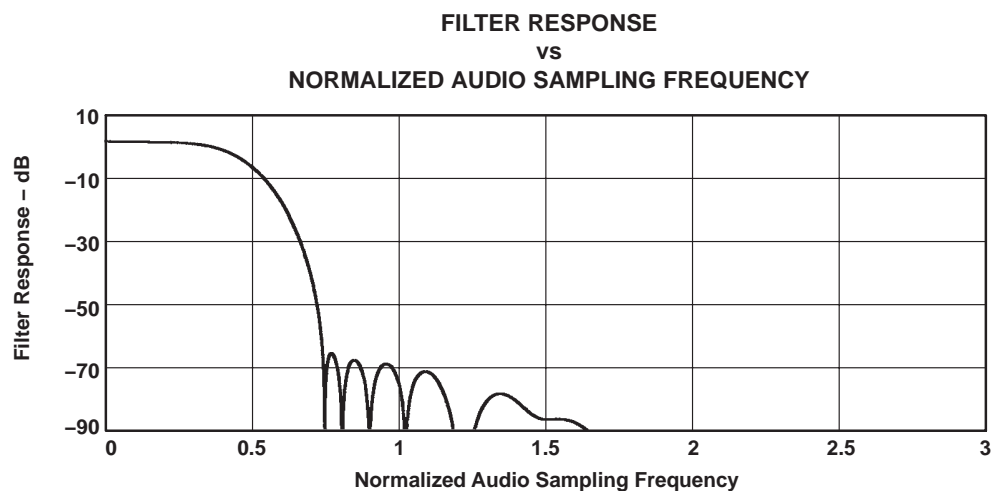
Figure 3-17. ADC Digital Filter Response 3: USB Mode Only
