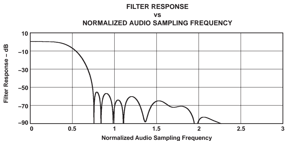
Figure 3-25. DAC Digital Filter Response 3: USB Mode Only
