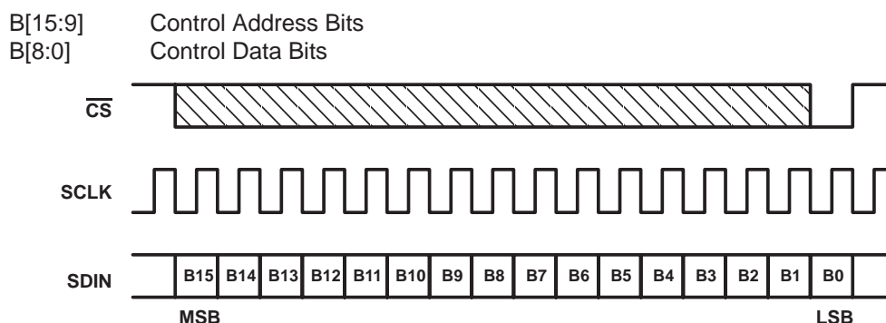
Figure 3–1. SPI Timing
