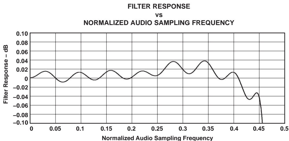
Figure 3-20. DAC Digital Filter Ripple 0: USB Mode
