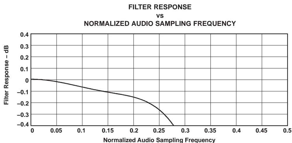
Figure 3-26. DAC Digital Filter Ripple 3: USB Mode Only
