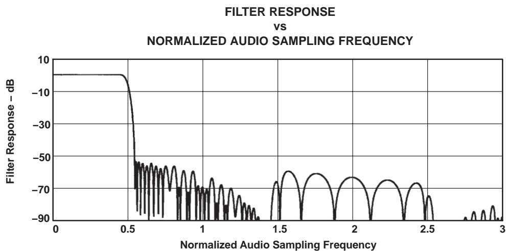
Figure 3-19. DAC Digital Filter Response 0: USB Mode
