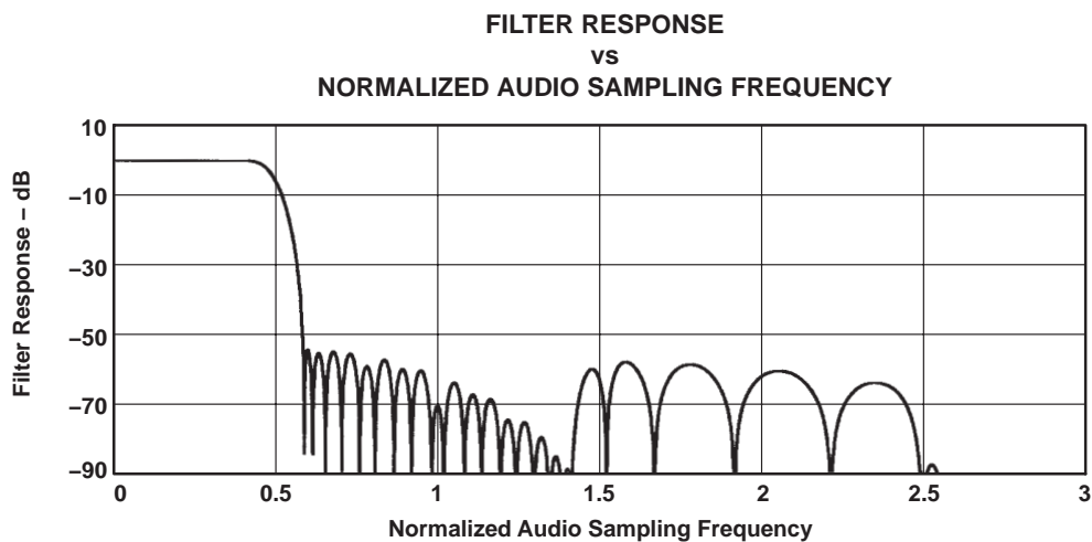
Figure 3–21. DAC Digital Filter Response 1: USB Mode Only
