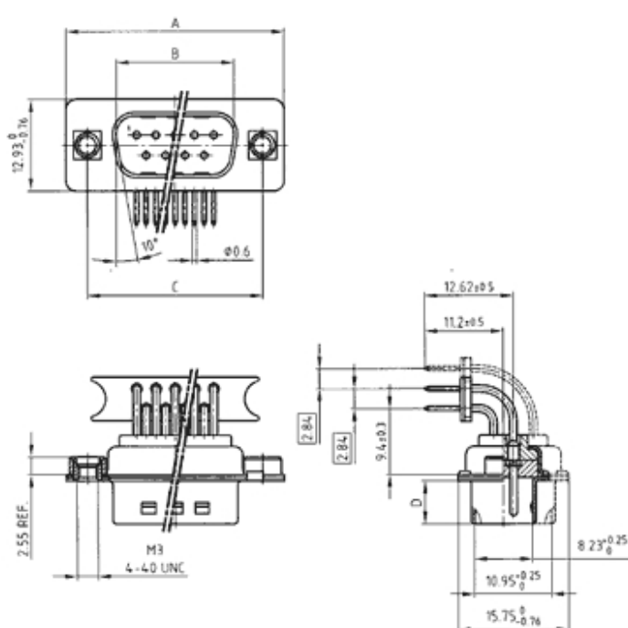
Plug connector
