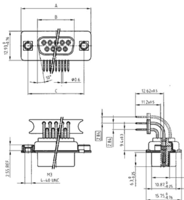
Socket connector
