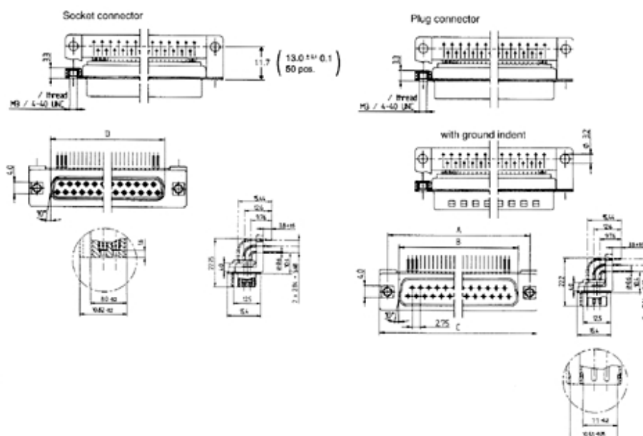
Socket connector:
