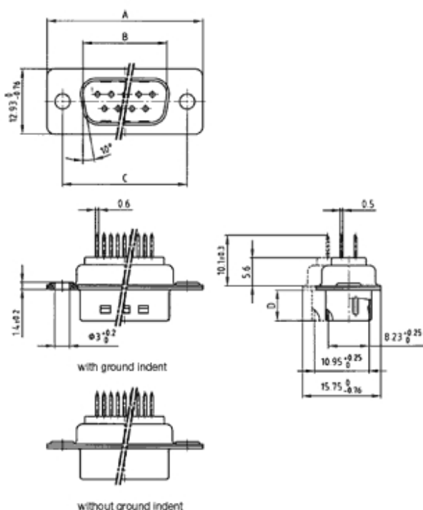
Plug connector
