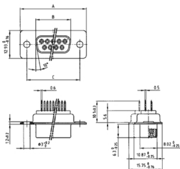
Socket connector
