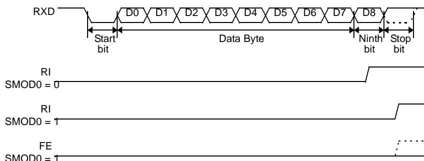
Figure 23. UART Timing in Modes 2 and 3
