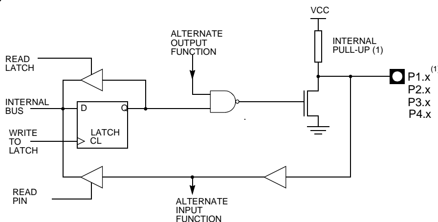
Figure 1. Ports Structure
