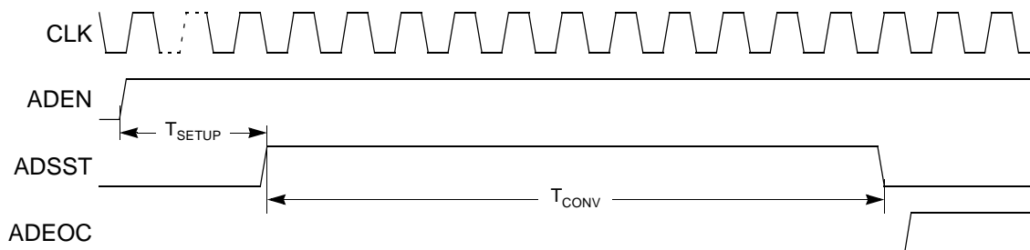
Figure 53. Timing Diagram
