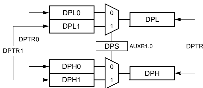
Figure 11. Dual Data Pointer Implementation
