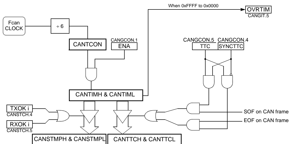
Figure 44. Block Diagram of CAN Timer
