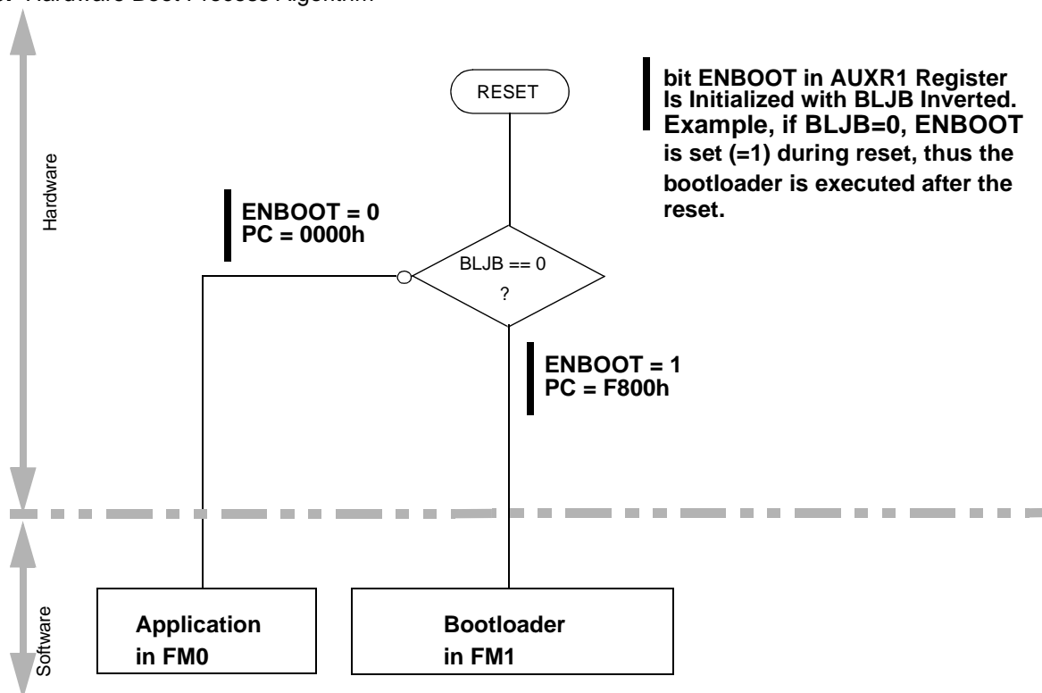
Figure 19. Hardware Boot Process Algorithm
