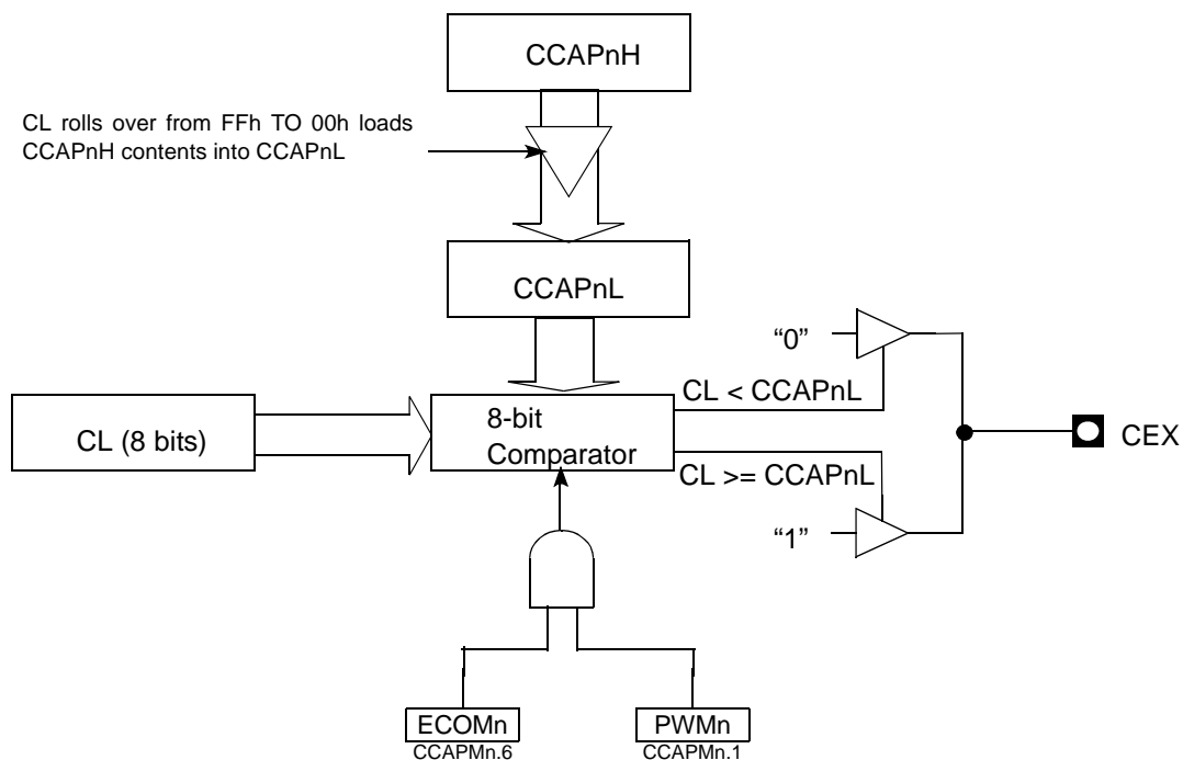
Figure 51. PCA PWM Mode
