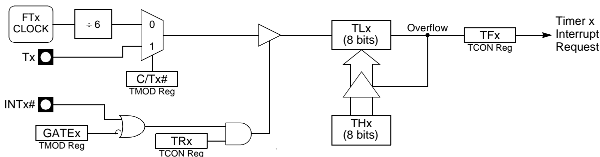
Figure 26. Timer/Counter x (x= 0 or 1) in Mode 2
