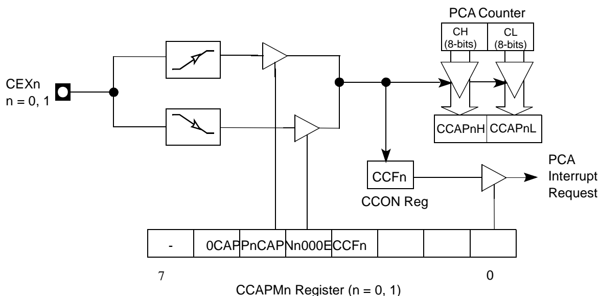
Figure 48. PCA Capture Mode
