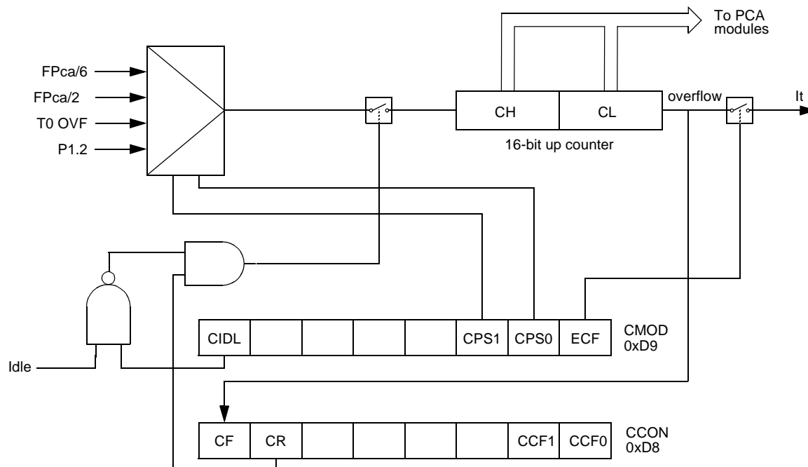
Figure 46. PCA Timer/Counter
