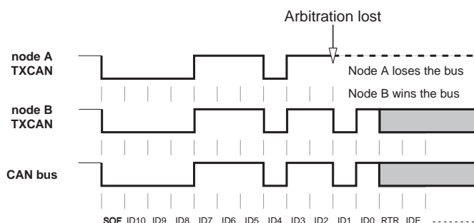
Figure 35. Bus Arbitration
