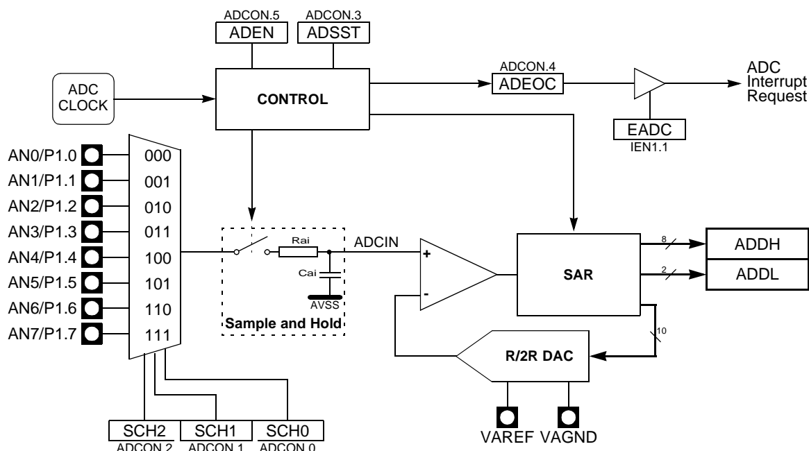
Figure 52. ADC Description
