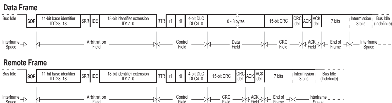
Figure 33. CAN Extended Frames
