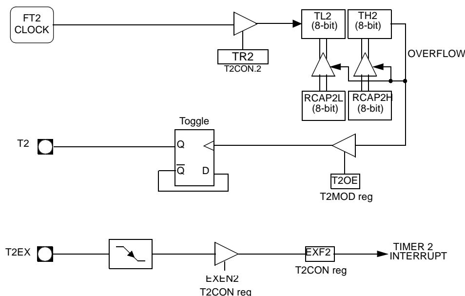
Figure 30. Clock-Out Mode
