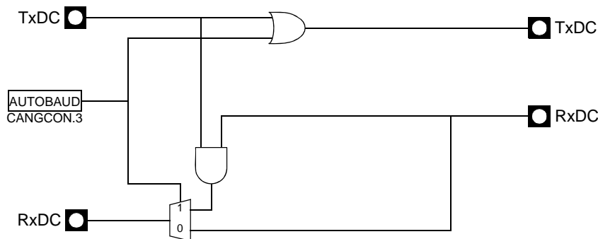
Figure 45. Autobaud Mode
