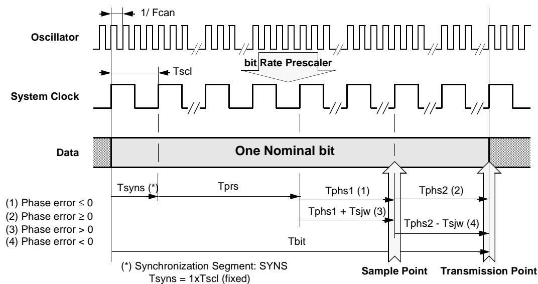
Figure 41. General Structure of a bit Period
