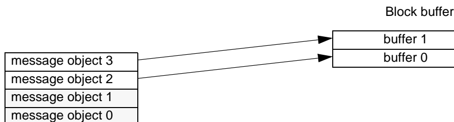
Figure 38. Buffer Mode
