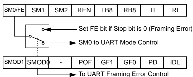
Figure 21. Framing Error Block Diagram
