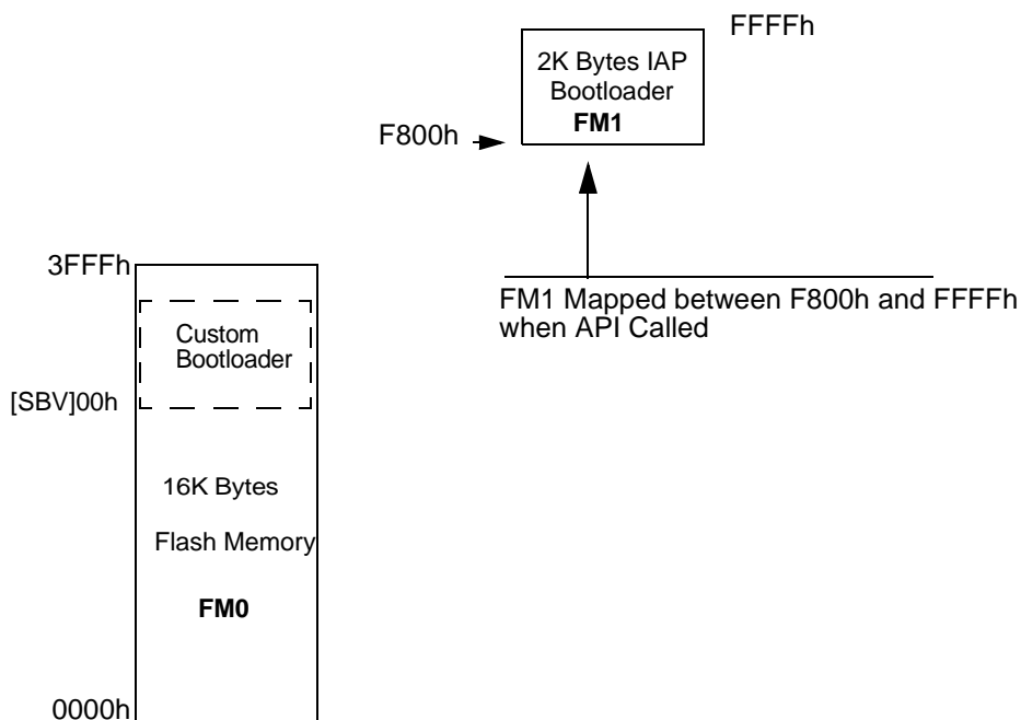
Figure 18. Flash Memory Mapping
