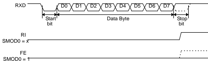
Figure 22. UART Timing in Mode 1
