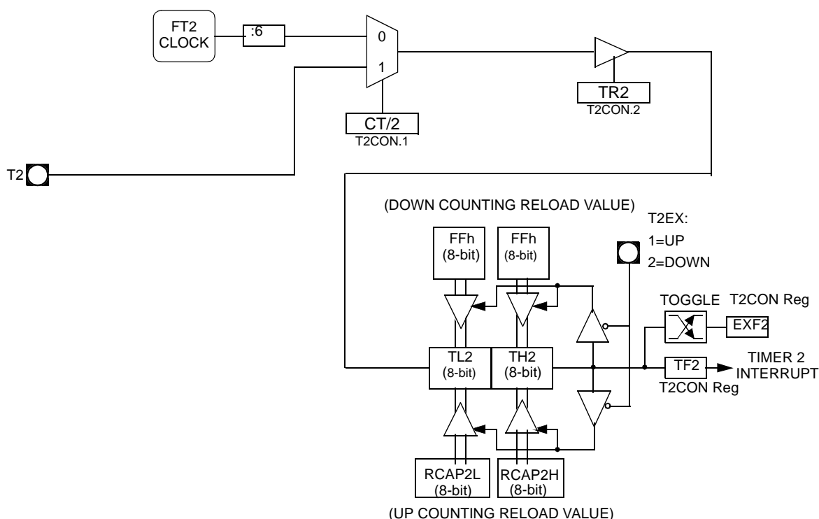
Figure 29. Auto-Reload Mode Up/Down Counter See section "Clock"
