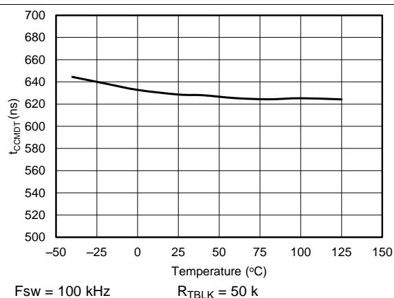
Figure 10. CCM Dead Time vs Temperature
