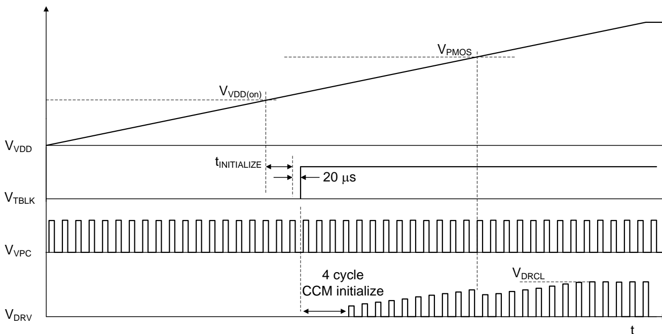
Figure 13. Start-Up Operation
