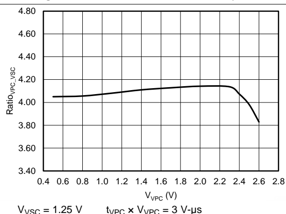
Figure 6. VPC-to-VSC Ramp-Gain Ratio vs VPC Voltage
