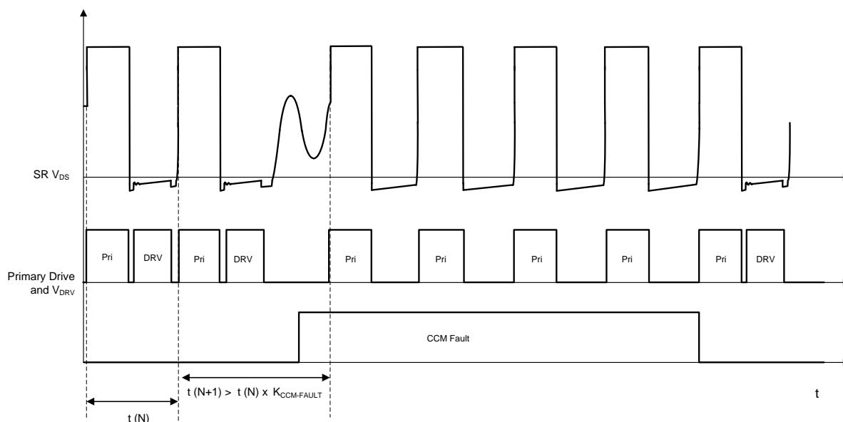
Figure 20. CCM Cycle-Fault Behavior, CCM Operation
