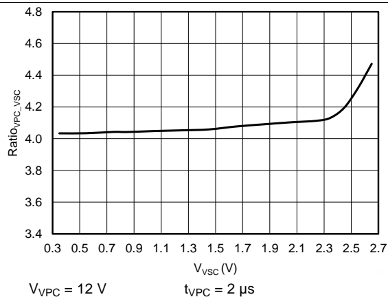
Figure 7. VPC-to-VSC Ramp-Gain Ratio vs VSC Voltage
