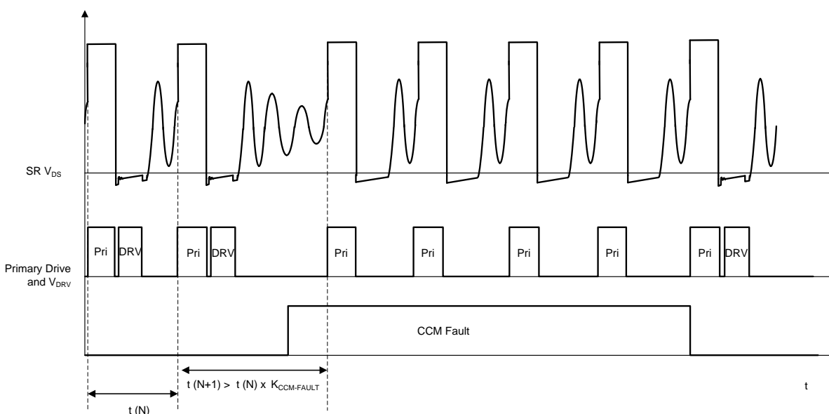
Figure 21. CCM Cycle-Fault Behavior, DCM Operation
