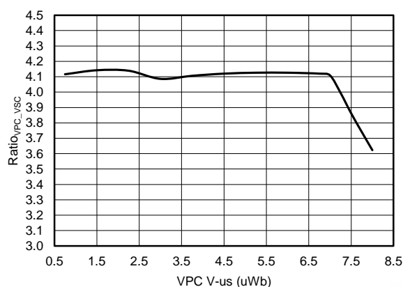
Figure 16. Ratio VPC_VSC vs VPC V- \mu s
