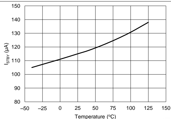
Figure 2. Standby Current vs Temperature
