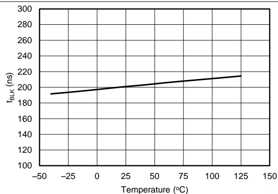
Figure 8. VPC Blanking Time vs Temperature (minimum setting)
