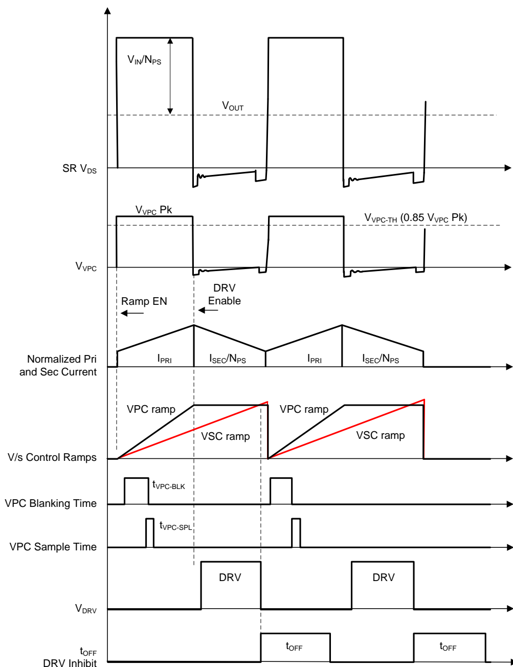
Figure 15. Operation in CCM
