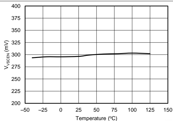
Figure 4. VSC Enable Threshold vs Temperature
