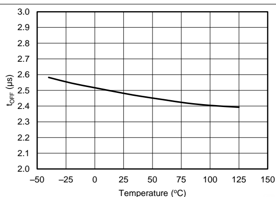
Figure 12. DRV Minimum Off Time vs Temperature
