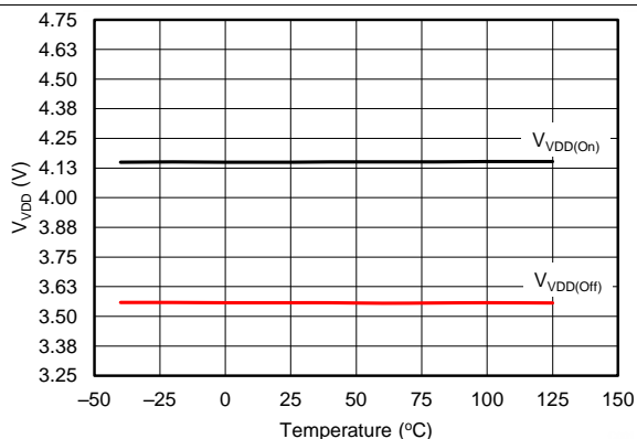
Figure 1. VDD Turn-On and Turn-Off Threshold vs Temperature
