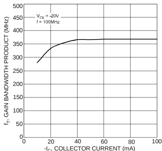
Fig. 13 Typical Gain-Bandwidth Product vs. Collector Current (2907A)
