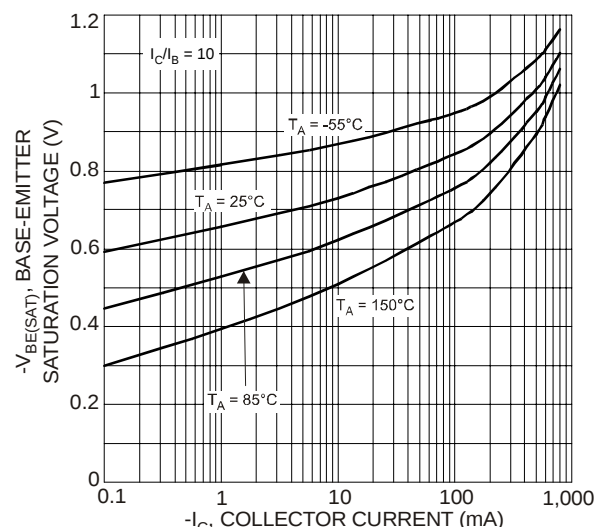
Fig. 11 Typical Base-Emitter Saturation Voltage vs. Collector Current (2907A)
