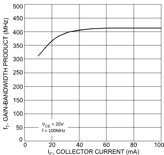
Fig. 7 Typical Gain-Bandwidth Product vs. Collector Current (2222A)
