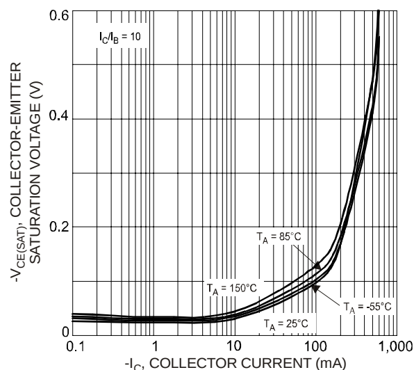
Fig. 9 Typical Collector-Emitter Saturation Voltage vs. Collector Current (2907A)
