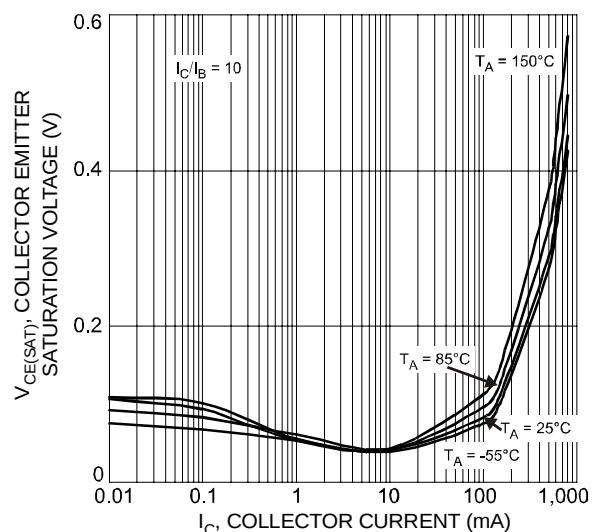
Fig. 3 Typical Collector Emitter Saturation Voltage vs. Collector Current (2222A)
