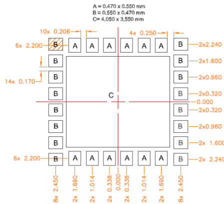
PCB Solder Mask Pattern
