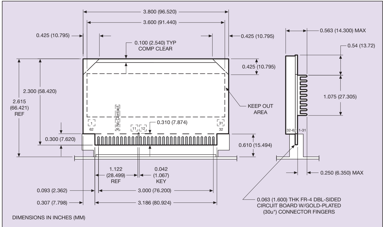
Figure 1: Mechanical Drawing
