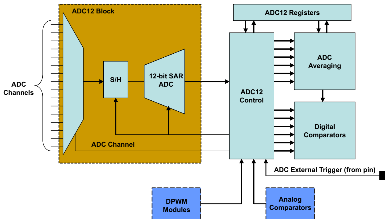
Figure 6-19. ADC12 Control Block Diagram
