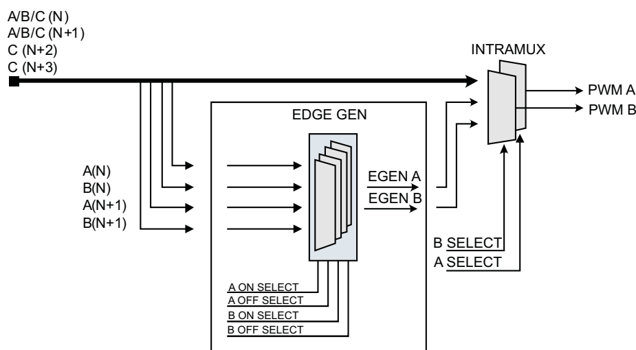
Figure 6-10. Edge Gen/Intra Mux
