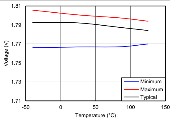
Figure 5-12. BP18 Voltage vs Temperature
