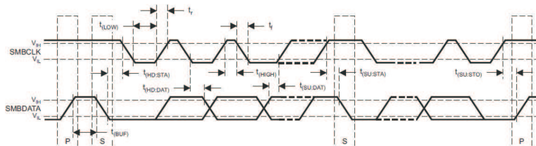
Figure 5-1. I 2 C/SMBus/PMBus Timing Diagram
