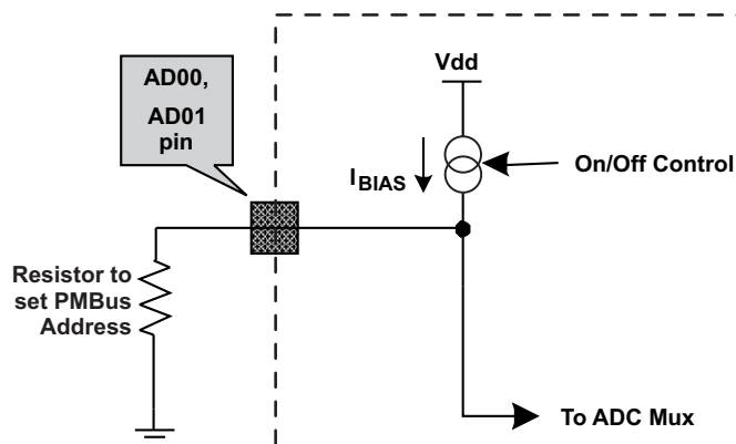
Figure 6-18. PMBus Address Detection Method
