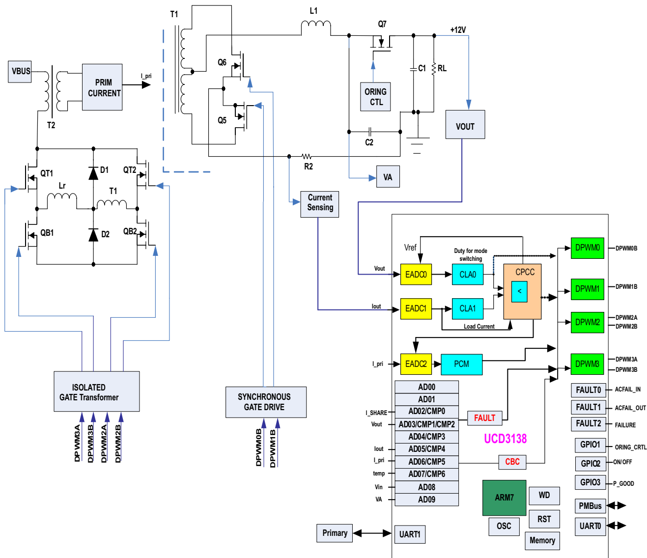
Figure 7-1. Phase-Shifted Full-Bridge
