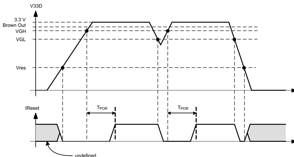
Figure 5-4. Power-On Reset (POR) and Brown-Out Reset (BOR)
