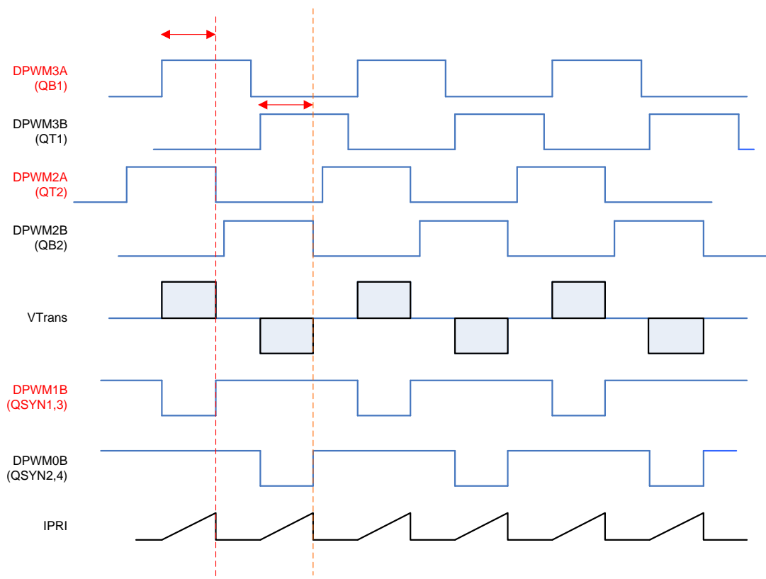
Figure 6-6. Phase Shifted Full Bridge
