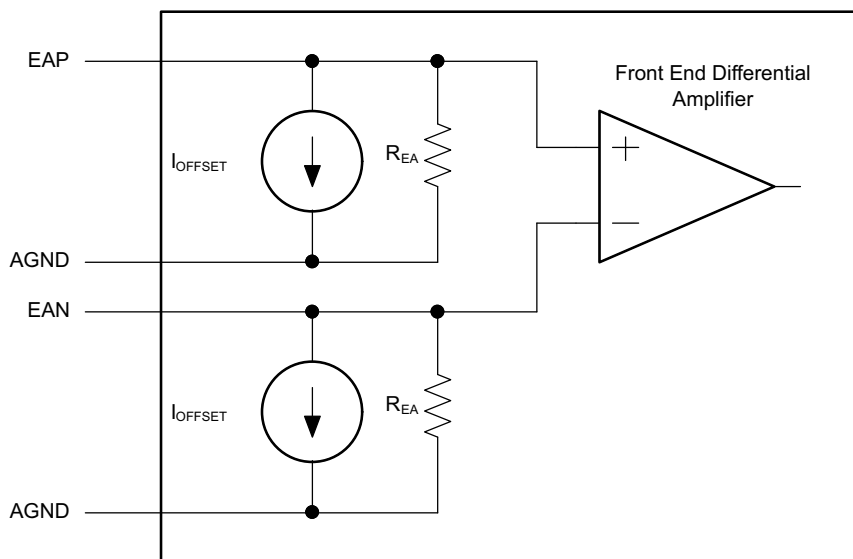
Figure 5-5. Input Stage of EADC Module
