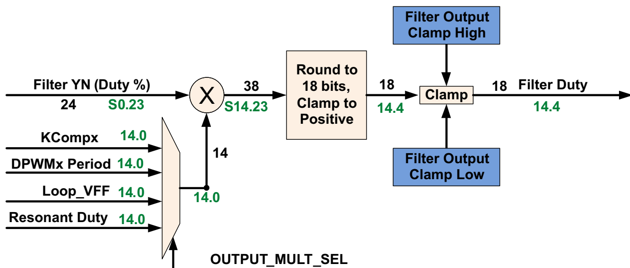
Figure 6-14. Resonant Mode
