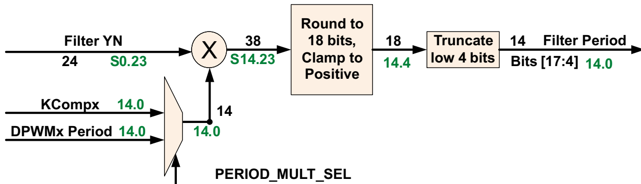
Figure 6-13. Final Section for the Filter
