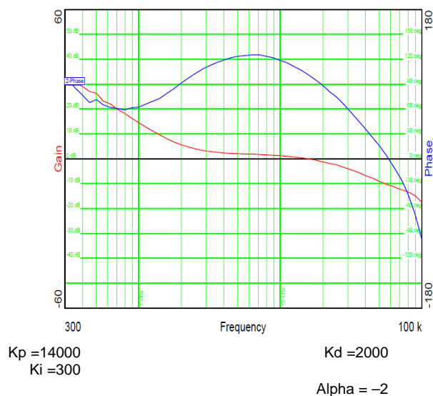
Figure 7-12. Bode Plot
