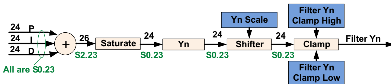
Figure 6-12. Output Section of the Filter
