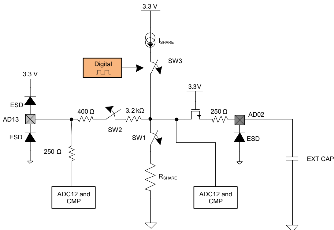
Figure 6-21. Simplified Current Sharing Circuitry
