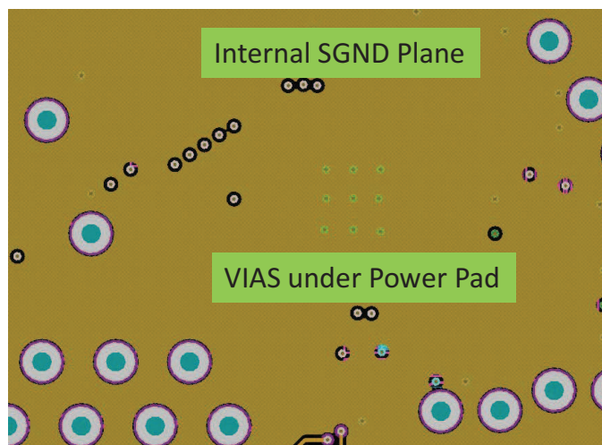
Figure 7-14. UCD3138A Layout Example, Internal Plane
