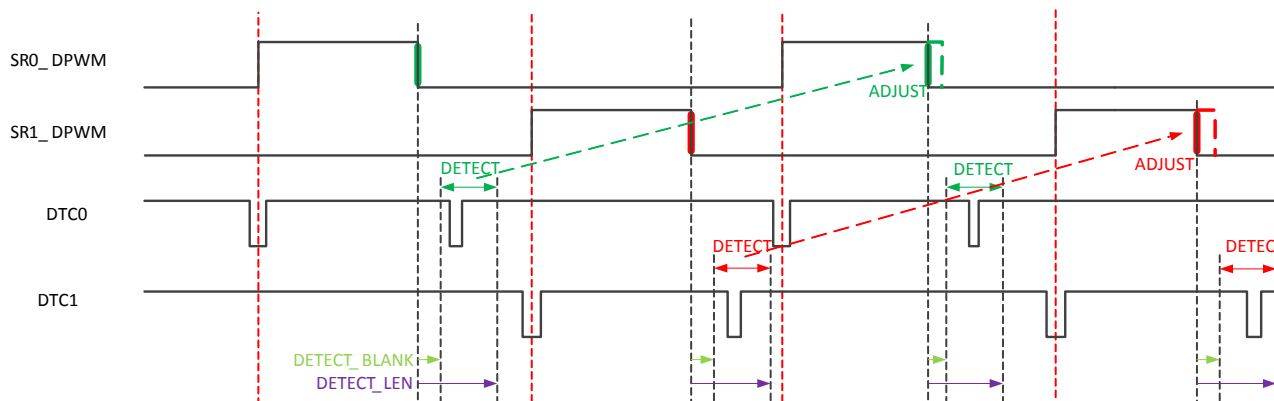
Figure 5-9. Timing Diagram of the DTC Interface
