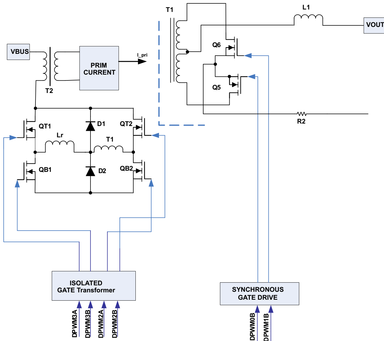
Figure 7-2. Schematic – PSFB Power Stage
