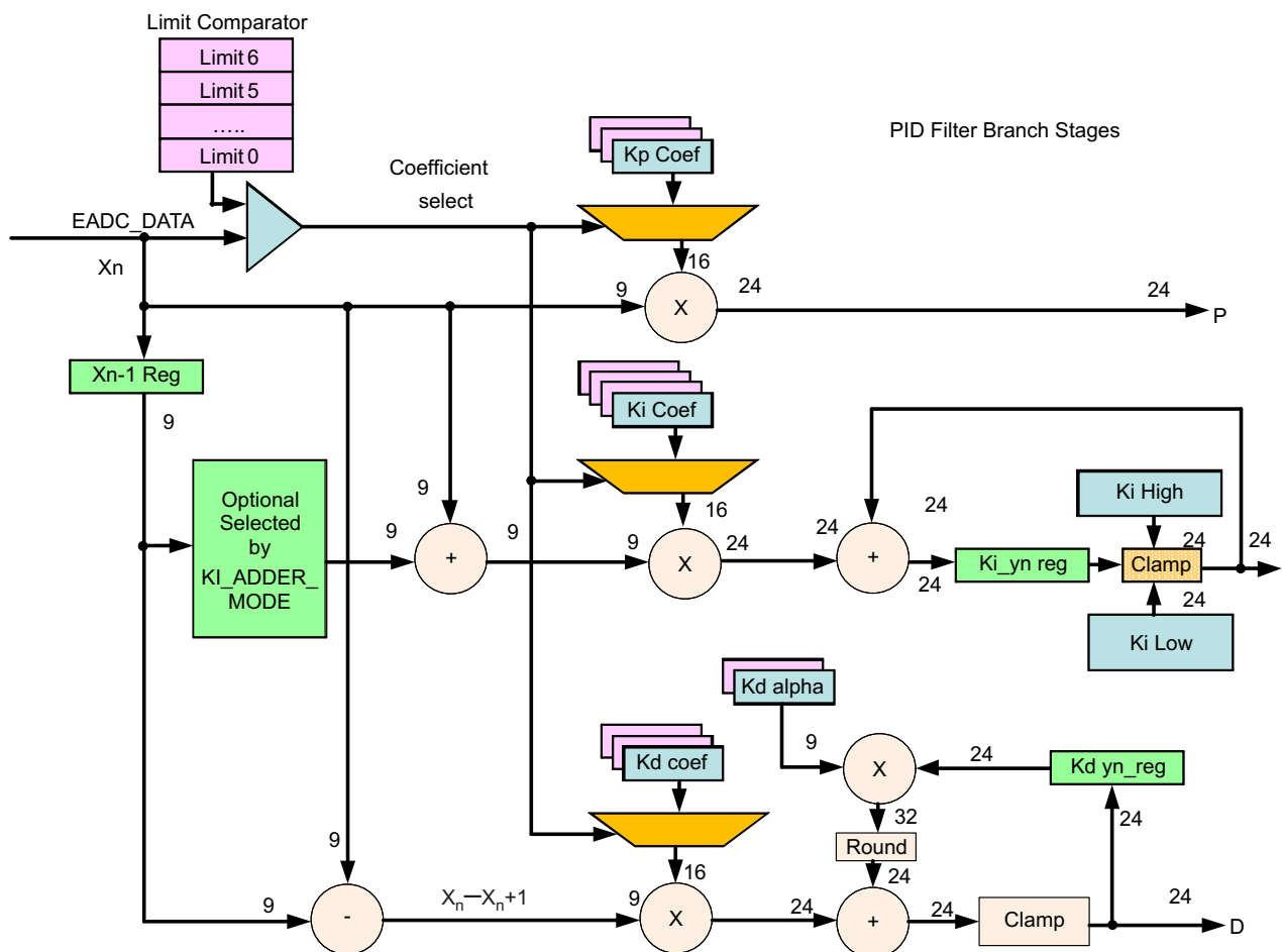
Figure 6-11. First Section of the Filter
