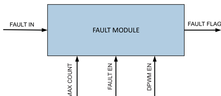
Figure 6-15. Fault Module
