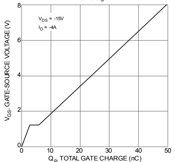
Figure 12 Gate-Charge Characteristics
