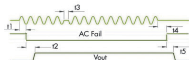
Mains AC Fail Signal
