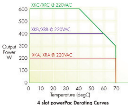
XKA/XKB/XKC and XRA/XRB/XRC @ 220VAC Derating
