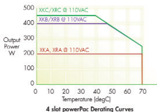
XKA/XKB/XKC and XRA/XRB/XRC @ 110VAC Derating
