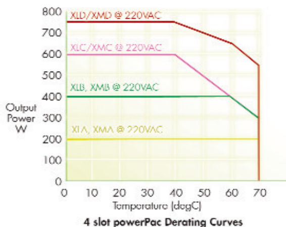
XLA/XLB/XLC/XLD and XMA/XMB/XMC/XMD @ 220VAC Derating
