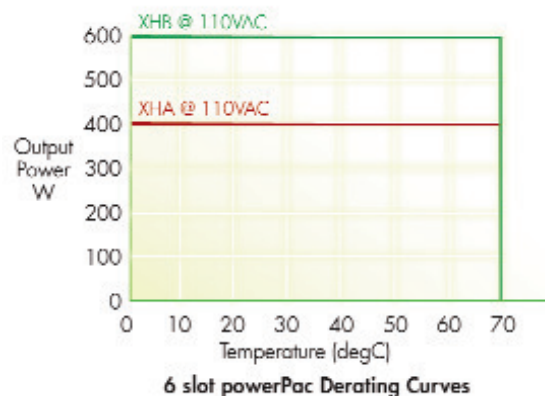
XHA/XHB @ 110VAC Derating
