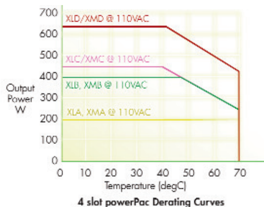
XLA/XLB/XLC/XLD and XMA/XMB/XMC/XMD @ 110VAC Derating
