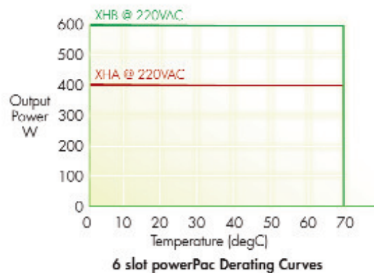
XHA/XHB @ 220VAC Derating
