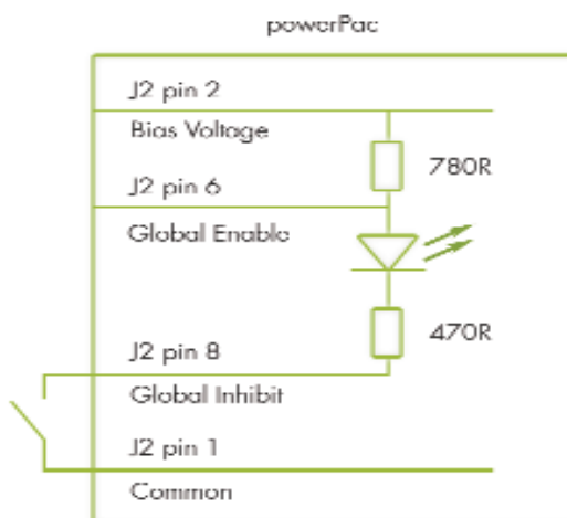
Global Inhibit Using Bias Supply Voltage
