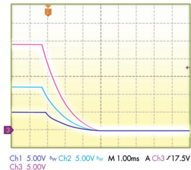
Output powerMod Shutdown
