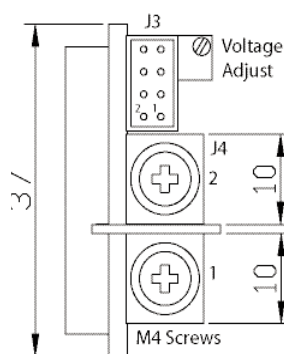
J4 Connector : M4 Screw
