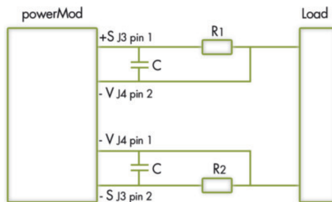
Remote Sense of Output Voltage
