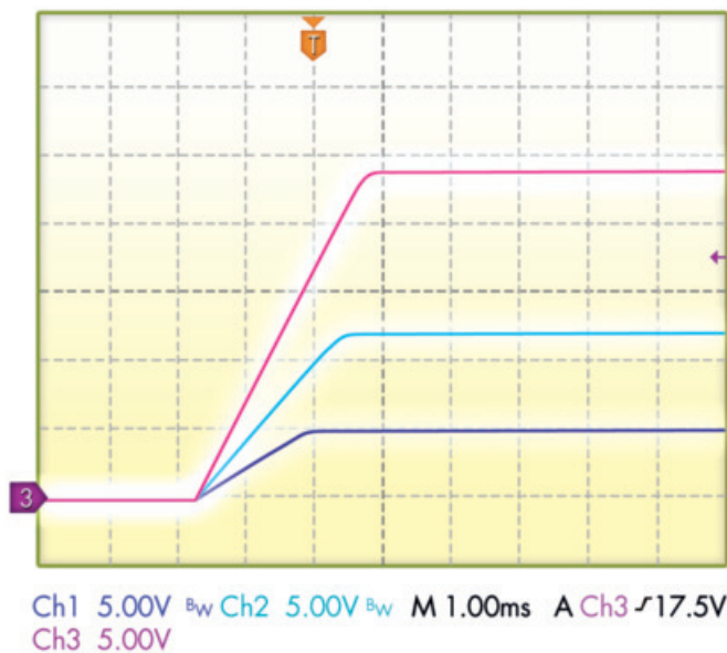
Output powerMod Start-Up
