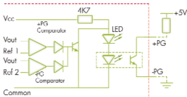
Output powerMods Power Good Signal
