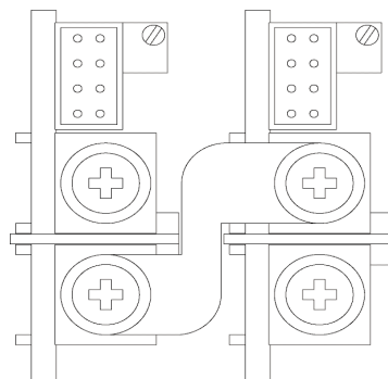
Series Connection of powerMods
