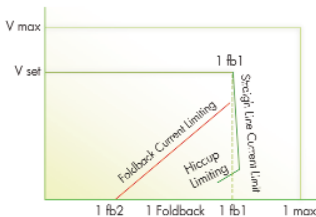
Current Limit Characteristics
