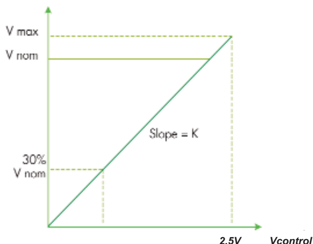
Remote Output Voltage Adjustment of powerMods
