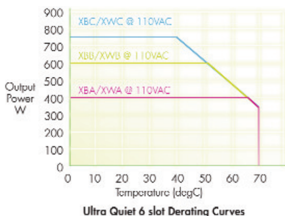
XBA/XBB/XBC and XWA/XWB/XWC @ 110VAC Derating
