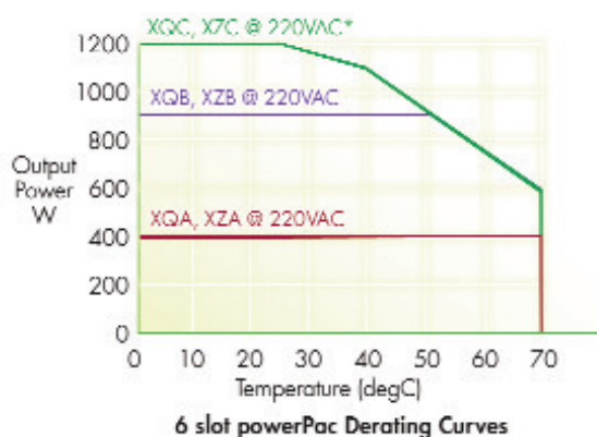
XQA/XQB/XQC and XZA/XZB/XZC @ 220VAC Derating
