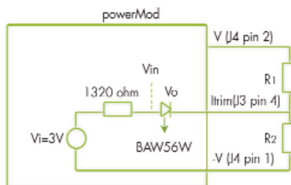
Foldback Current Limit
