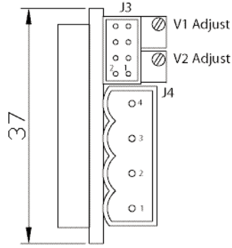
J4Connector : Camden 9200/4A
