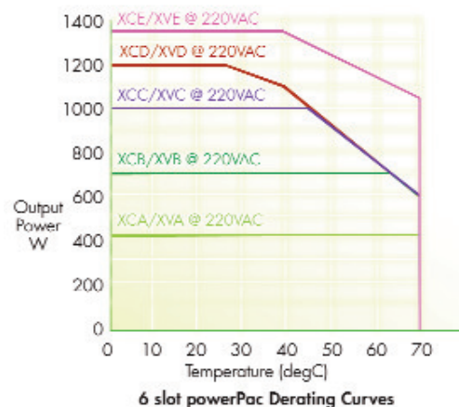
XCA/XCB/XCC/XCD/XCE and XVA/XVB/XVC/XVD/XVE Derating @ 220VAC Derating
