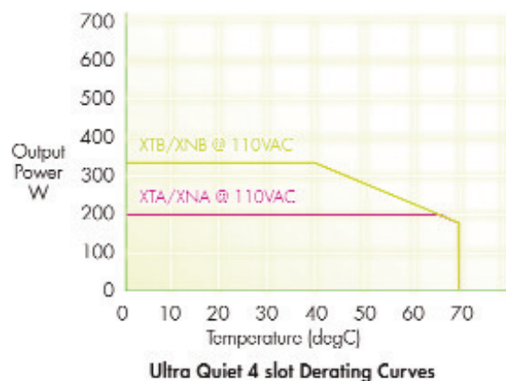
XTA/XTB and XNA/XNB @ 110VAC Derating
