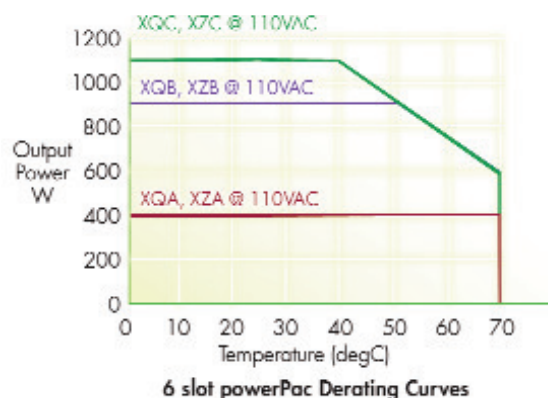
XQA/XQB/XQC and XZA/XZB/XZC @ 110VAC Derating
