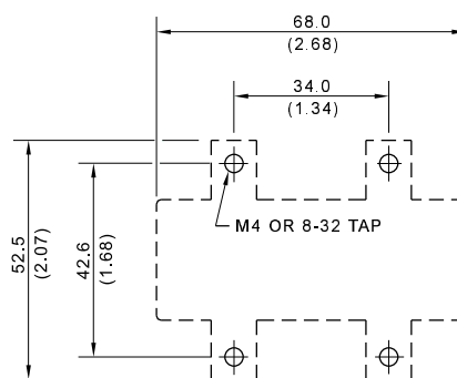
MOUNTING DETAIL
